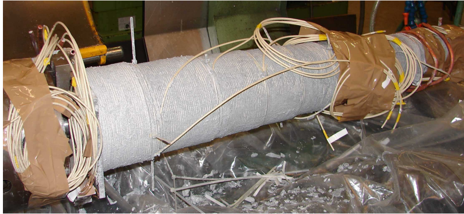
Figure 3.2: The Zeeman slower while being wound. One can see the layer structure of the coils. The cables are held in place using a cement mixed with silicon carbide, which gives a grey color. On the right one can see the end of the two parallel water cooling tubes which are below the coils.
