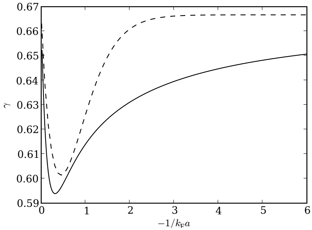
Figure 5.9: The effective polytropic exponent \gamma as a function of the inverse gas parameter. The solid line is calculated from the fit in figure 5.8, while the dashed line is the mean-field BCS theory.
