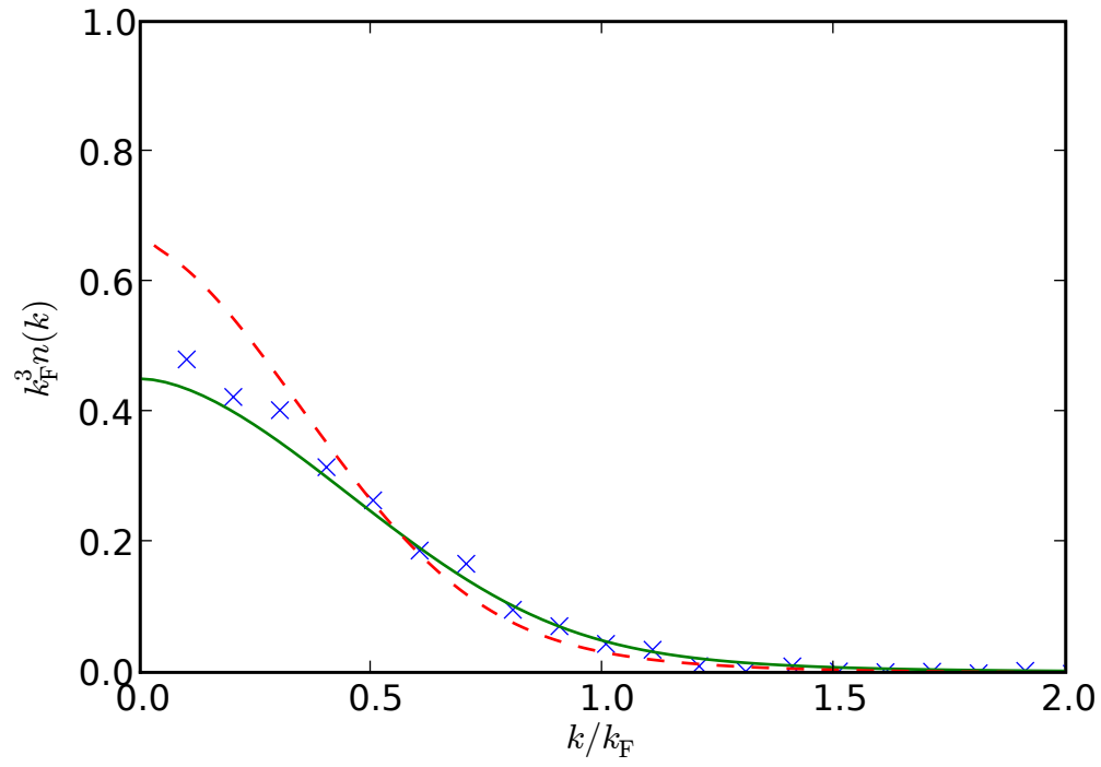
Figure 5.3: The momentum distribution of a gas at the unitarity limit. The crosses are the inverse Abel transform of the cloud. The solid curve is the distribution at zero temperature as calculated in section 5.1.1. The dashed line is the prediction by Astrakharchik et al. [70]. The data is averaged over three images.
