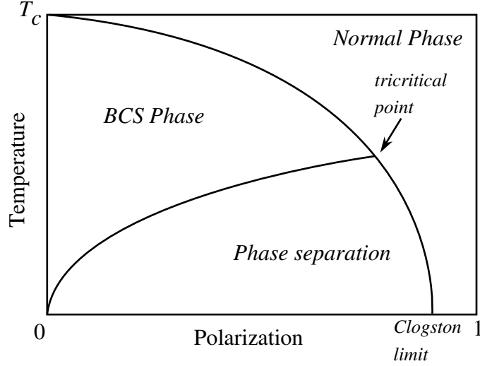
Figure 5.21: A sketch of the phase diagram of a spin-polarized Fermi gas. The temperature is given in the unit of the transition temperature T_c for a polarized gas. A polarization of 1 means that all spins are oriented in the same direction, while 0 means that the gas is completely depolarized. Figure adopted from reference [136]
