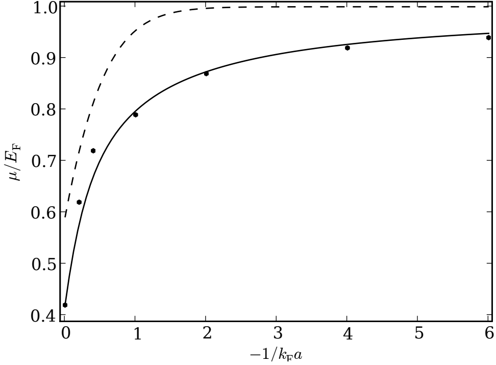
Figure 5.8: The chemical potential as a function of the inverse gas parameter in the homogeneous case. The points are Monte-Carlo simulations from reference [79], the solid line is the fit presented in reference [112], while the dashed line is the prediction from mean-field BCS theory.
