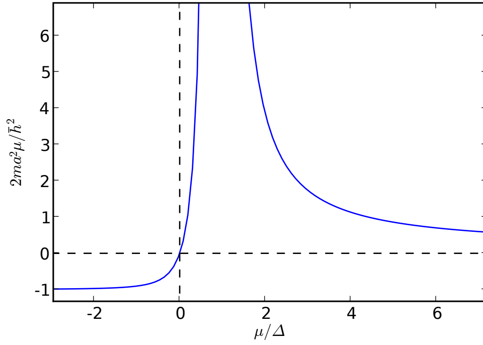
Figure 5.1: An illustration of the gap equation. We present the normalized chemical potential as a function of the ratio x_0 of the chemical potential and the gap. The left branch corresponds to the BEC side of the resonance, while the right one corresponds to BCS.
