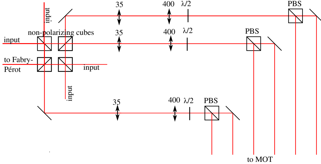
Figure 3.6: The optical setup for the MOT
