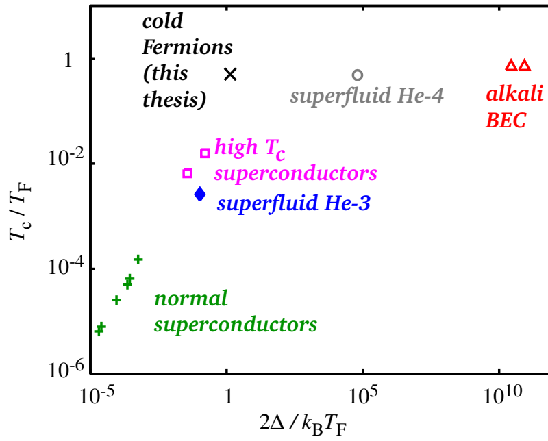
Figure 1.1: The critical temperature and the pair binding energy of various superfluid fermionic systems. The two bosonic systems in the graph (He-4 and alkali BEC) are considered as composite boson consisting of the ionic core and the valence electron for alkali, and of the ionic core and one electrons for He-4. Our experiments are marked as \times . Figure modified from reference [10].
