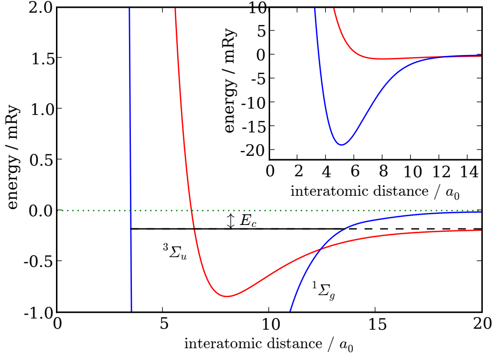
Figure 2.3: The two scattering potentials involved in the Lithium-6 Feshbach resonances. ^3\Sigma_u is the triplet, and ^1\Sigma_g is the singlet state. The singlet state contains bound states. The triplet state can be shifted using a magnetic field. Here, we show a shift down such that the dissociation energy of the triplet potential coincides with the bound state in the singlet state. This is what happens close to a Feshbach resonance. The binding energy E_c is not to scale, in reality the bound state is so close to dissociation that the difference would not be visible in this graph. The insert shows the overall picture at zero magnetic field. Data adopted from references [51,52].
