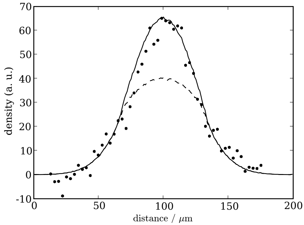
Figure 5.16: Simulation of a molecular Bose-Einstein condensate. The solid line is the atomic density, the dashed line is the thermal cloud. The points are experimental data. The data is taken at k_F a \approx 1 .
