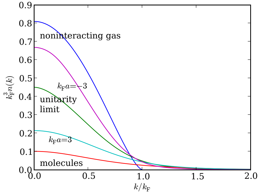
Figure 5.2: The calculated momentum distributions in a harmonic trap. The curves are normalized to \int_0^\infty n(k)k^2 dk = 1 . The areas under the curves are not equal as the number of atoms is proportional to the density multiplied by the surface of the sphere with radius k . k_F is the Fermi wave vector calculated for the noninteracting gas.
