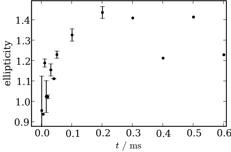
Figure 5.13: The ellipticity of the cloud for various times in the magnetic field at the unitarity limit. The expected ellipticity for long expansion times is 1,4. This is the same dataset as figure 5.6, the error bars are calculated in the same way.
