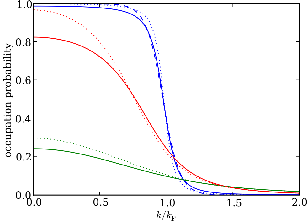
Figure 2.8: The momentum distribution in a homogeneous gas in the different limits of BCS theory. On the top the BCS limit, k_F a = -1 . The dashed line shows a Fermi gas at the critical temperature for comparison. The center line is the unitarity limit ( 1/k_F a = 0 ) and the bottom line is the BEC limit ( k_F a = 1 ). The dotted lines are the predictions from Astrakharchik et al. [70].
