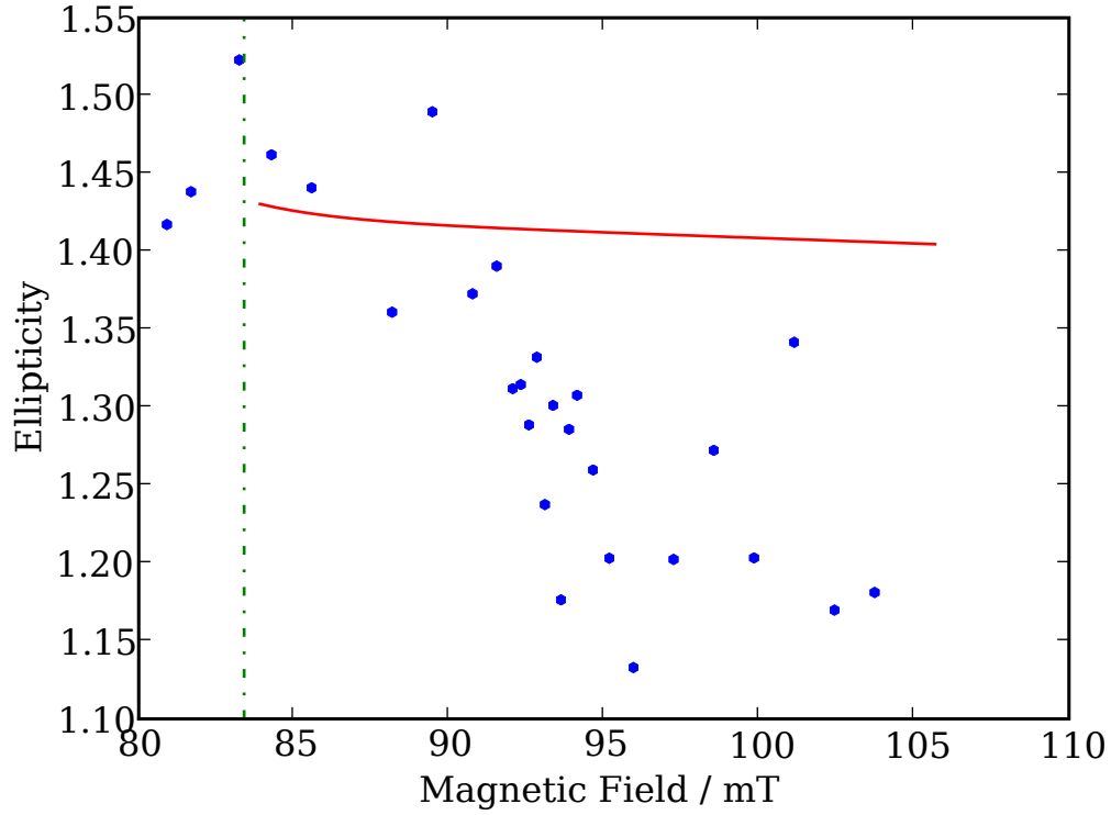
Figure 5.11: Ellipticity of the gas after expansion in a magnetic field on the BCS side of the crossover. The temperature was determined with a two-dimensional Fermi fit to be T = 0,17T_F . The solid line shows the theoretical expectation, as calculated in section 5.3. The dashed line marks the position of the Feshbach resonance. While at the resonance the experimental points agree with a superfluid hydrodynamic expansion, they leave this function in a step-like manner. We average images at same magnetic fields before applying the gaussian fit.
