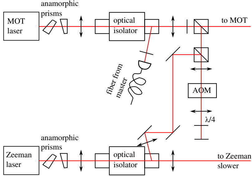
Figure 3.7: The principal optical setup for the lasers on the experimental table. Note that the ^7\text{Li} principal Zeeman laser is not injected by the MOT lasers, but directly from the fiber via the AOM.
