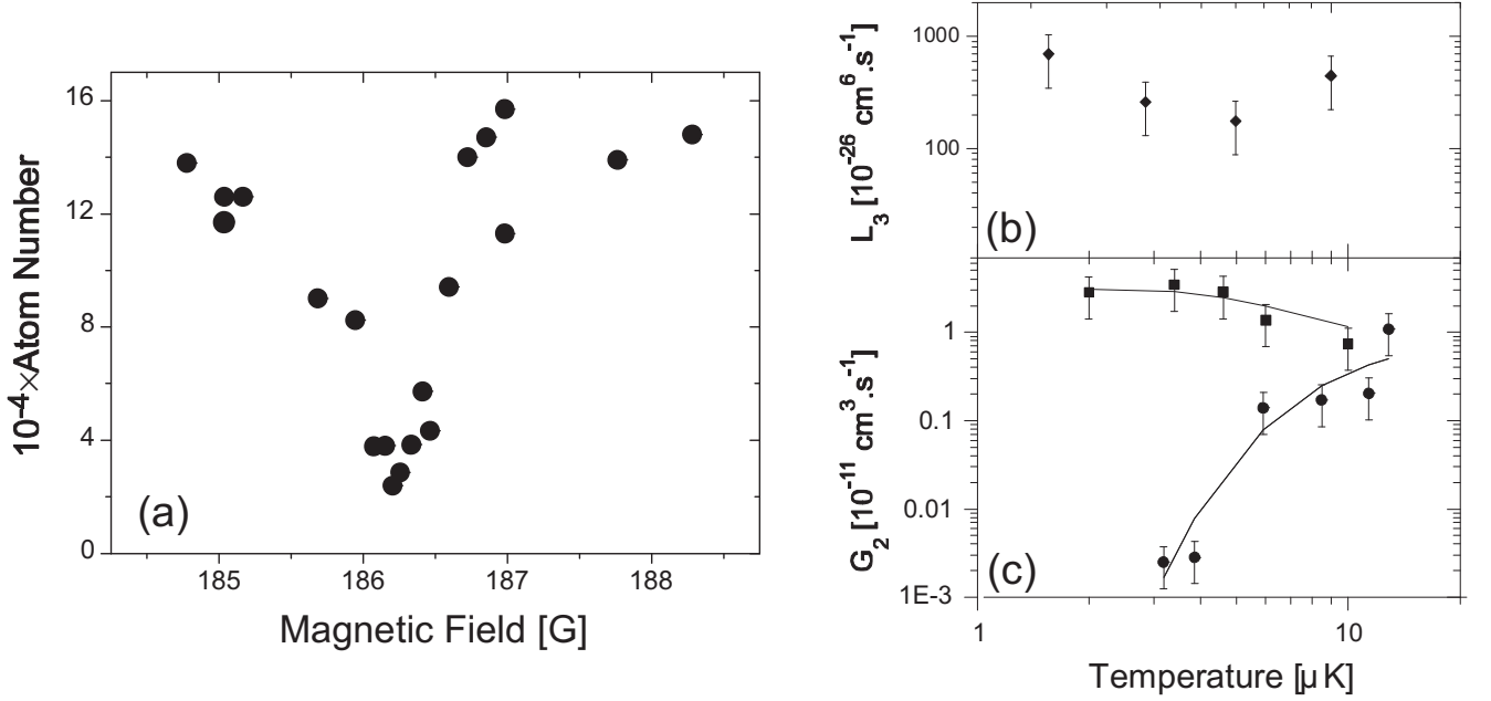
FIG. 3: (a) Atom number vs. magnetic field B_{0,f} after a 50 ms wait for atoms in the spin mixture (1/2, -1/2) at T \sim 14 \mu\text{K} . The sharp drop close to B_0 \sim 186 G over a range \simeq 0.5 G is the signature of the p-wave Feshbach resonance predicted by theory. (b) (resp. (c)) Variations of 3-body (2-body) loss rates vs temperature at the Feshbach resonance. (b): \blacklozenge : atoms in the Zeeman ground state |f = 1/2, m_f = 1/2\rangle , B_{0,f} \sim 159 G. (c): \blacksquare : atoms polarized in |f = 1/2, m_f = -1/2\rangle , B_{0,f} \sim 215 G. \bullet : mixture |f = 1/2, m_f = 1/2\rangle + |f = 1/2, m_f = -1/2\rangle , B_{0,f} \sim 186 G. In both cases, the full line is a fit to the data using prediction of Eq. 3 with the magnetic field as the only fitting parameter.
