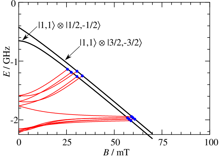
Figure 5.17: The bound states and Feshbach resonances for a mixture of ^7\text{Li} and ^6\text{Li} . This figure corresponds to figure 2.4, which describes the same situation in ^6\text{Li} only. We only searched for the resonances between the lowest Zeeman states, as in such a gas inelastic collisions are suppressed. Image taken from reference [122]
