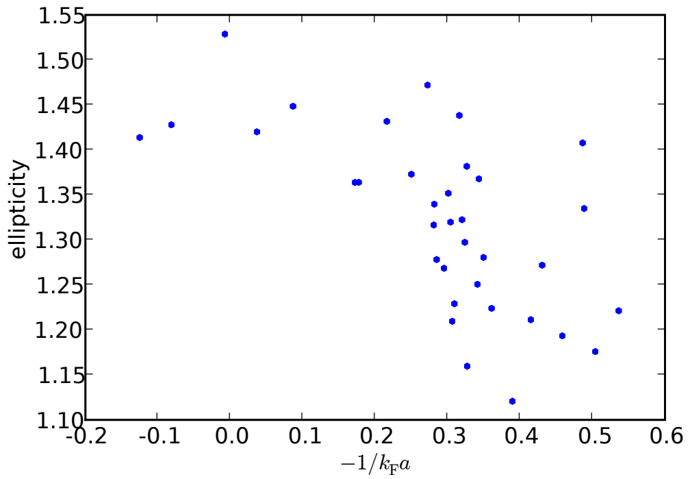
Figure 5.12: The ellipticity as a function of -1/k_F a . The step happens at a gas parameter of about k_F a = 0,3 . Since the temperature is about T = 0,17T_F (see text), this is consistent with the predicted transition temperature in figure 2.9.
