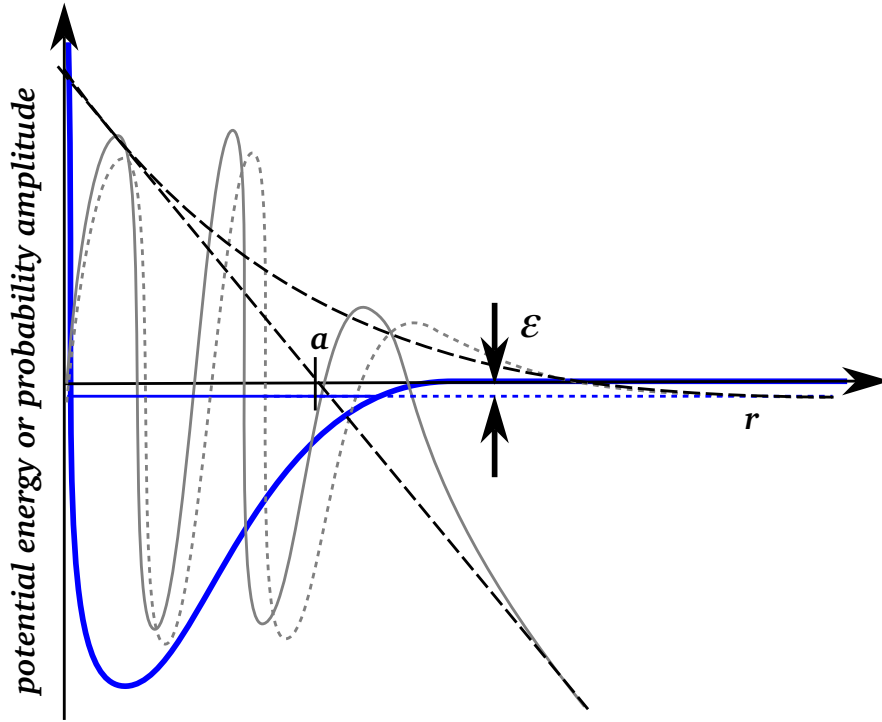
Figure 2.1: A sketch of a shape resonance. A bound state with binding energy \epsilon is located just below the dissociation energy in the potential (thick solid line), its wave function is drawn as a grey dotted line, it exponentially decays for large distances r . The free state symbolized by the solid line is very close to the bound state, for large distances it will become a sine function with a very long wavelength. One extends the bound state exponential and free state sine function to the origin, as if there was no potential, drawn as dashed lines, and connects them there (The lower dashed line is not a straight line but the beginning of a sine with a very long wavelength). The distance where this extended wave function crosses zero is the scattering length a .
