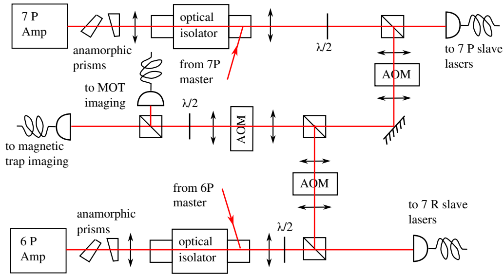
Figure 3.8: The setup of the MOT amplifiers and imaging lasers. The ^7\text{Li} principal and ^6\text{Li} principal beams are generated in a saturated absorption spectroscopy, tunable via an acousto-optic modulator. This is the beams entering into this picture. Two amplifiers give enough power for both the MOT slave lasers and the imaging. Three AOMs guarantee that there is always two AOMs switching the light, as stray light would be evil, and enable us to switch the to isotopes independently.
