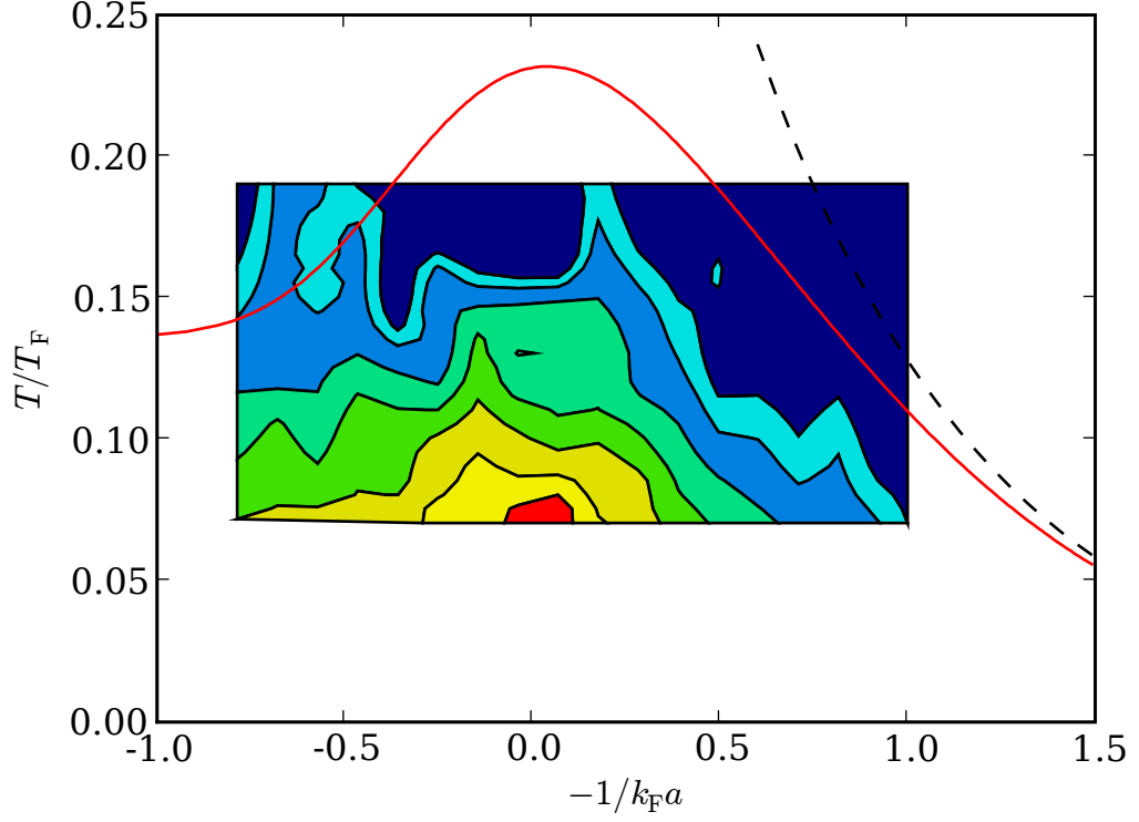
Figure 2.9: The transition temperature in the BEC-BCS crossover (solid line). The data in the background is a measurement taken in ^{40}\text{K} of the condensate fraction. Above the curve the gas is in the normal state, while we have a superfluid phase below. We note that there is no phase transition between a superfluid BEC on the left side and BCS superfluidity on the right. Both theory and data is by Chen et al. [27]. The colors correspond to a condensate fraction between 0 (dark) and 15,5% (bright). The curve is higher than the data since they could not measure a condensate fraction below 1%. The dashed line shows the transition temperature usually used to describe superconductivity in metals, it is the temperature below which pairing begins.
