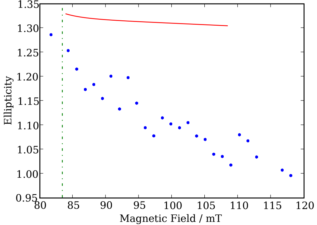
Figure 5.14: The ellipticity in the crossover at higher temperatures: here T = 0,3T_F . The step has disappeared. The residual ellipticity is lower than its superfluid counterpart in figure 5.11
