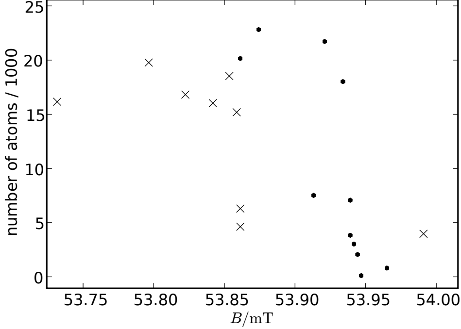
Figure 5.19: An example for the measurement of the position of a heteronuclear Feshbach resonance. Here we show the most interesting of the four resonances, where the position changed with the ramping speed. The magnetic field was ramped in 1 s from lower values, 47,5 mT for the crosses, 53,7 mT for the dots, to the value indicated in this graph. One sees a sharp loss of atoms.
