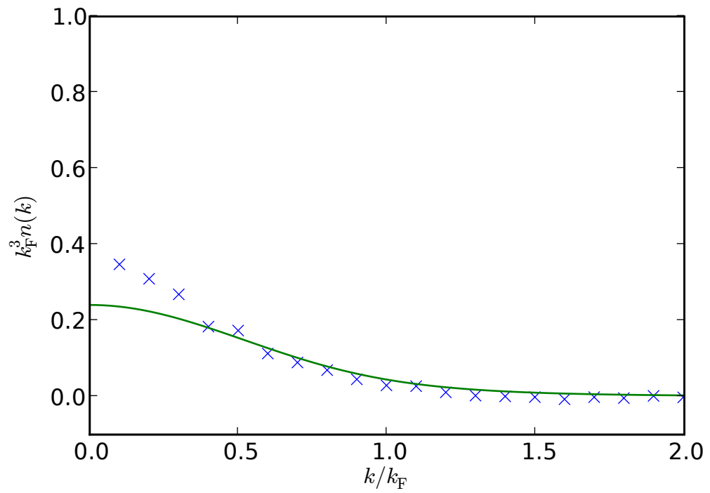
Figure 5.4: The momentum distribution of a gas in the molecular regime. k_F a = 3 , with about 1.5 \cdot 10^5 atoms. The data (crosses) is averaged over three images. The solid line shows the theoretical predictions explained in the text.
