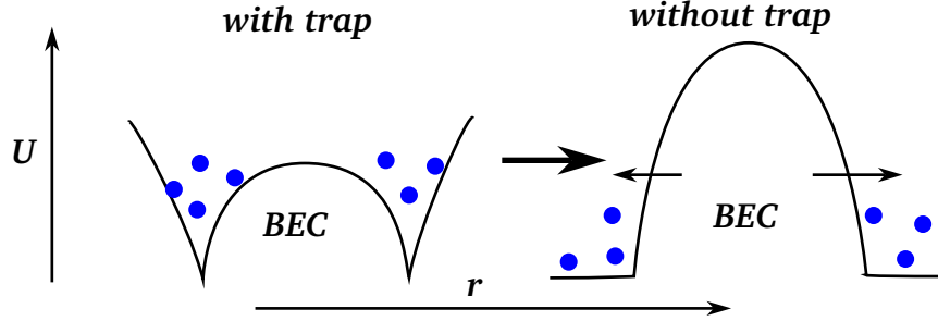
Figure 5.15: Illustration of the model used in the text. The points represent the thermal cloud. They are trapped in a potential created by the BEC before the trap is switched off, and pushed outwards afterwards by the expanding BEC.
