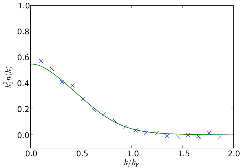
Figure 5.5: The momentum distribution of a gas on the BCS side of the resonance. k_F a = -3.5 , with about 1.5 \cdot 10^5 atoms, averaged over two images. The crosses are the experimental points, while the solid line shows the BCS predictions (see text).
