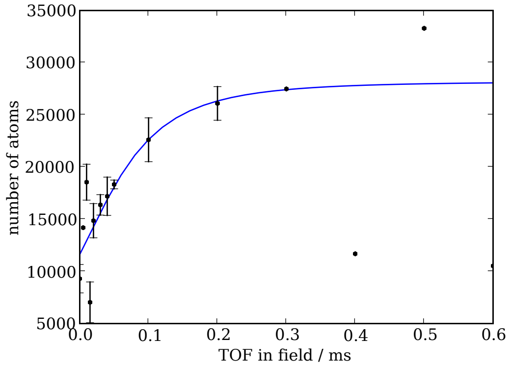
Figure 5.6: The number of detected atoms as function of the time of flight \tau in magnetic field at the unitarity limit. The error bars are one standard error, the points without error bars are single points, thus the error is not defined. The line is a fit with the Landau-Zener model described in the text.
