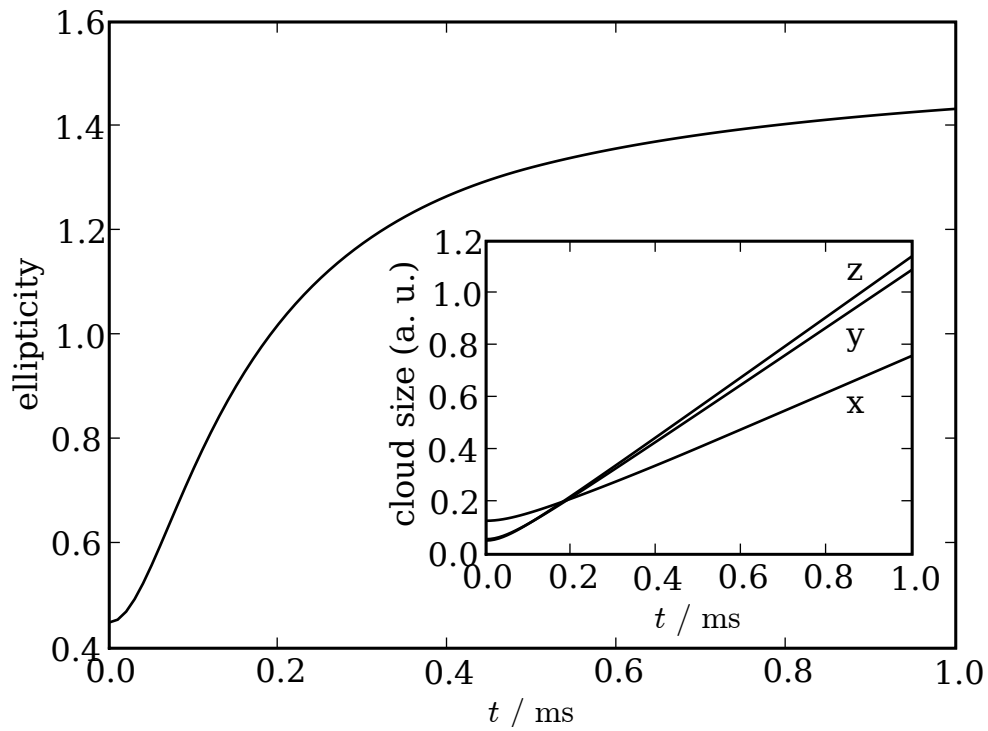
Figure 5.10: The ellipticity of an atomic cloud while expanding in a magnetic field. The parameters are the same as for the experiments which will be shown in the experimental section, namely in figure 5.11. The inset illustrates the behavior of the diameter of the three axes, the notation of the axis is described in the text.
