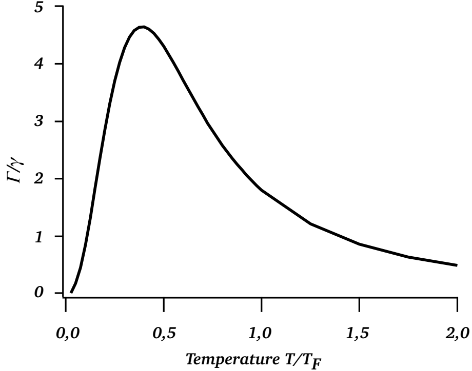
Figure 5.7: The correction factor between the typical scattering rate \gamma resulting from the calculations in the text and the real scattering rate \Gamma as a function of the temperature. The scattering rate decreases for high temperatures as does the scattering cross section. At low temperatures the Pauli exclusion principle reduces the scattering rate. This can decrease scattering down to values found in the noninteracting regime, but as the gas condenses at these low temperatures, it will become hydrodynamic. Figure taken from reference [106]
