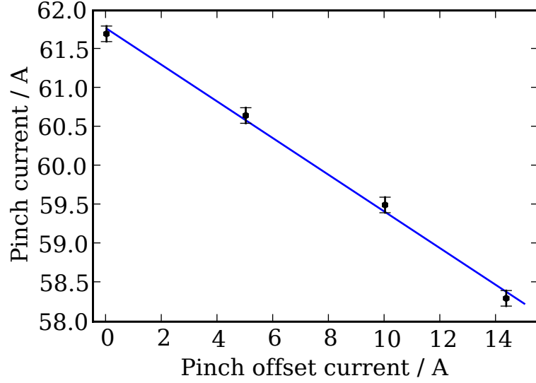
Figure 5.20: Calibration of the magnetic fields of the two coil systems. The points are the position of the p -wave resonance |1/2, 1/2\rangle + |1/2, 1/2\rangle . The fit of the points gives a calibration of I_{\text{pinch}} = 0,24 I_{\text{offset}} .
