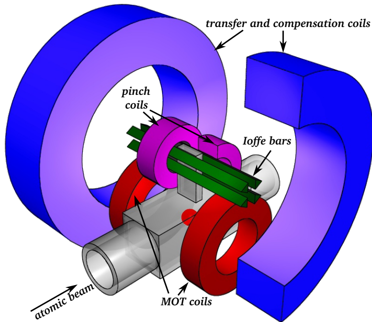
Figure 3.9: The magnetic coils setup.
