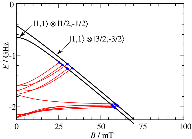
Figure 5.17: The bound states and Feshbach resonances for a mixture of ^7\text{Li} and ^6\text{Li} . This figure corresponds to figure 2.4, which describes the same situation in ^6\text{Li} only. We only searched for the resonances between the lowest Zeeman states, as in such a gas inelastic collisions are suppressed. Image taken from reference [122]
