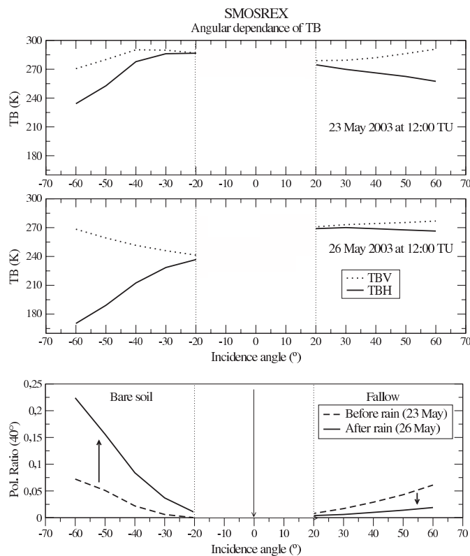
Fig. 8. Angular signature of the microwave signal on fallow and bare soil. Negative (−60° to −20°) and positive (20° to 60°) incidence angles correspond to bare soil (left) and fallow (right) respectively.
