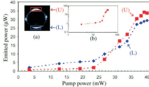
FIG. 3 (color online). Optical power of the upper (U) and lower (L) beam as a function of the pump power. Cavity-excitation detuning \delta = 0 . Inset (a) the zones over which the upper and lower emissions are, respectively, integrated are shown. Inset (b) log-log plot of the upper beam emission as a function of pump power.
