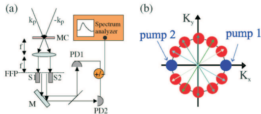
FIG. 1 (color online). (a) Experimental setup. Two pump beams \mathbf{k}_p and -\mathbf{k}_p are focused on the microcavity MC. The microcavity emission is collimated by a lens ( f = 50 mm). Two movable screens S1 and S2 placed in the far field plane (FFP) eliminate the transmitted pump beams. The upper part of the emission is detected by photodiode PD1, the lower part by photodiode PD2. The photocurrent sum and difference are then spectrally analyzed. (b) Representation in k space of the expected scattering processes. Correlated pairs are connected by arrows.
