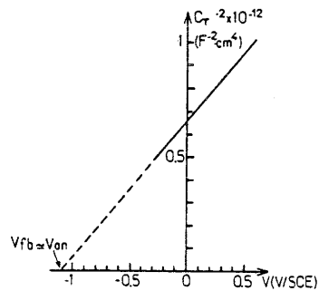
Fig. 13. Mott-Schottky graph for SrTiO 3 (pc).
