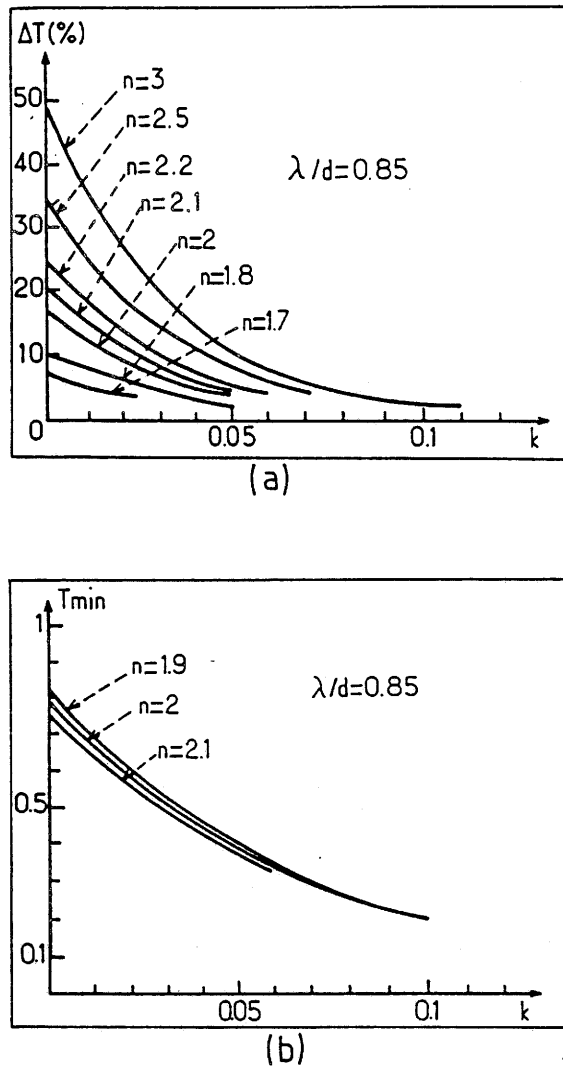
FIGURE 7 Theoretical curves \Delta T = f(k) , (a), and T_{\min} = f(k) , (b), for n = c^e and \lambda/d = c^e .
