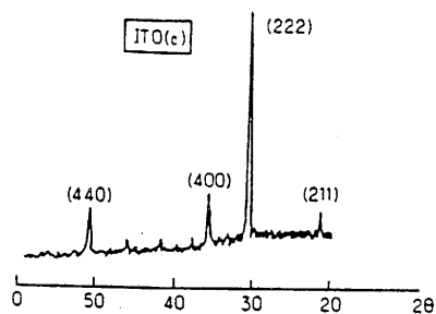
Fig. 1. X-ray diffraction patterns for ITO films deposited at room temperature (ITO (a)) and at 300^\circ\text{C} (ITO (c)).
