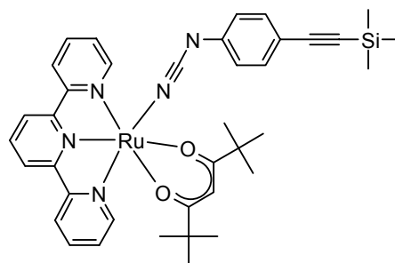
[Ru(tpy)(thd)(TMSepcyd)]
