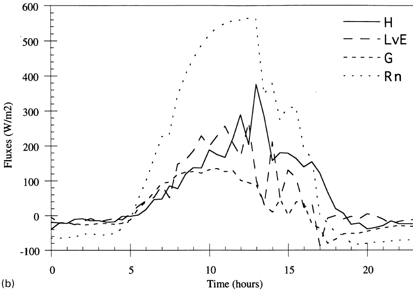
Fig. 2. (a) atmospheric forcing (air temperature, T_a ( ^{\circ}\text{C} ), relative humidity, hu (%), wind speed U_a ( \text{m s}^{-1} ), incoming solar R_g and long-wave R_a radiations ( \text{W m}^{-2} ) measured on 22 June 1991 (DOY 173); (b) surface energy budget (net radiation R_n , sensible heat flux H , latent heat flux L_v E and soil heat flux G ( \text{W m}^{-2} )) derived from measurements by the SAMER micrometeorological station on 22 June 1991 (DOY 173).
