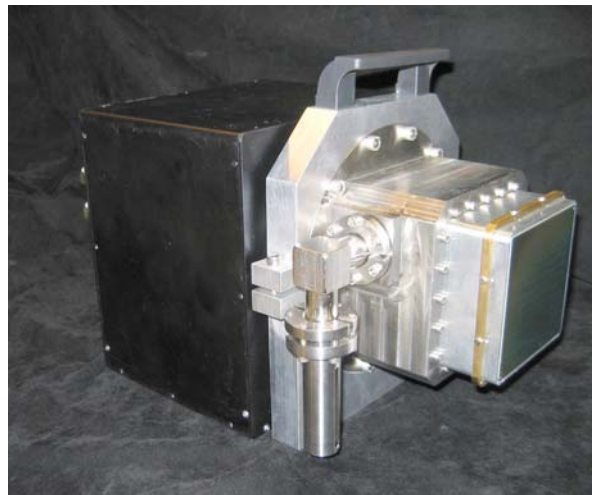
Figure 3.15. The ID17 taper optics FReLoN camera.
