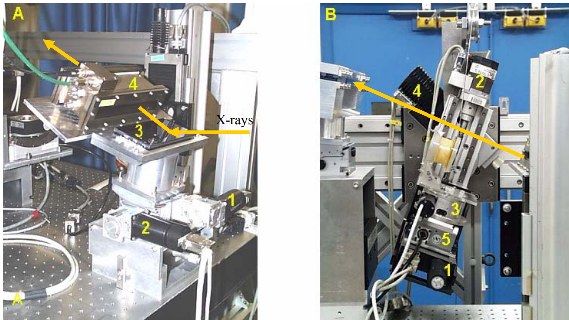
Figure 3.19. A) The pre-monochromator stage (n° 1, 2, 3) and the IC1 (n° 4). B) The sample stage (n° 1-5).
