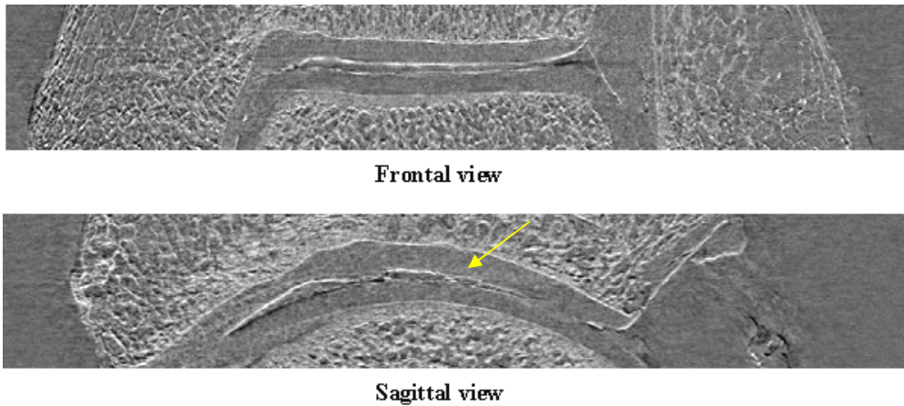
Figure 5.23. Lateral slices of the ankle constructed by ABI tomography acquisitions (details in the text).
