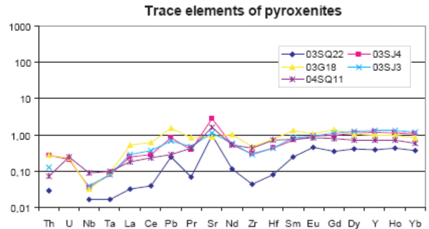
Figure 3.14b. Trace elements of pyroxenites. Normalized to primitive mantle (Sun and McDonough, 1989).
