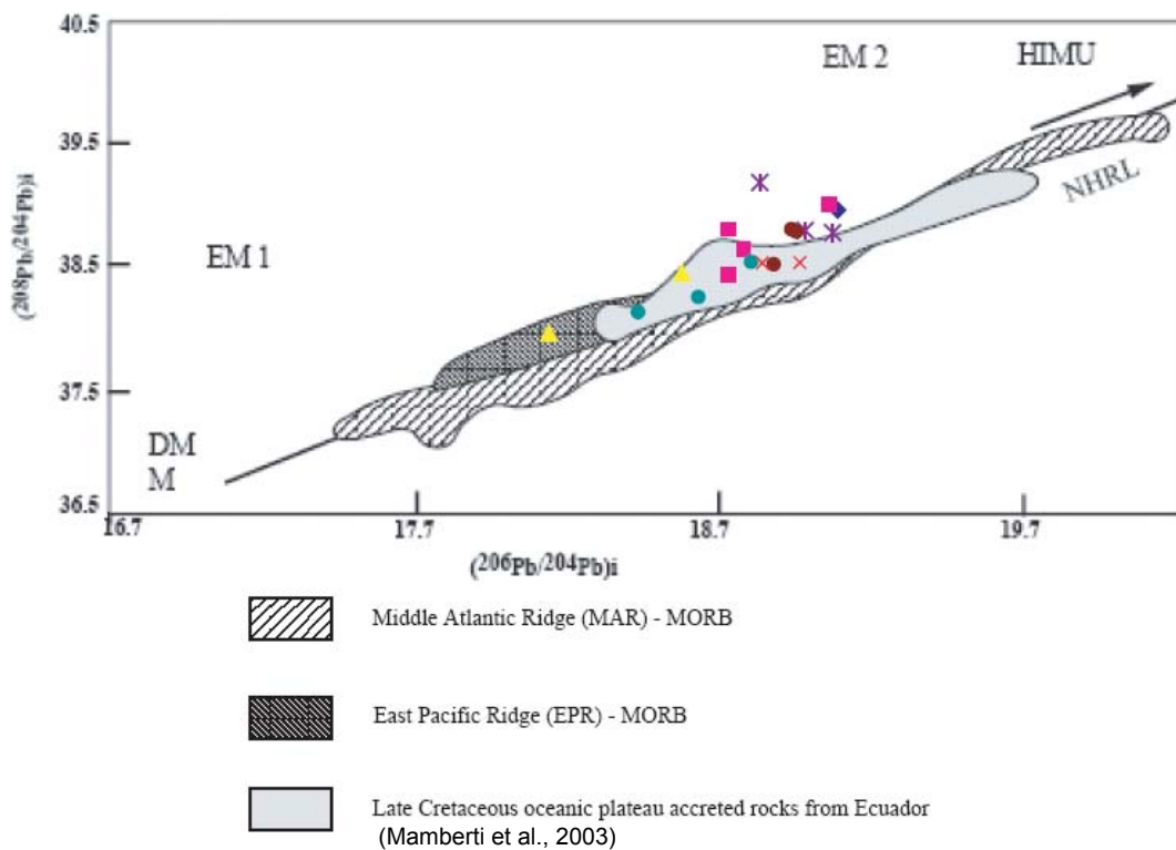
Figure 3.36b. (^{208}Pb/^{204}Pb)_i versus (^{206}Pb/^{204}Pb)_i for igneous, metamorphic and ultramafic rocks of Ecuador.
