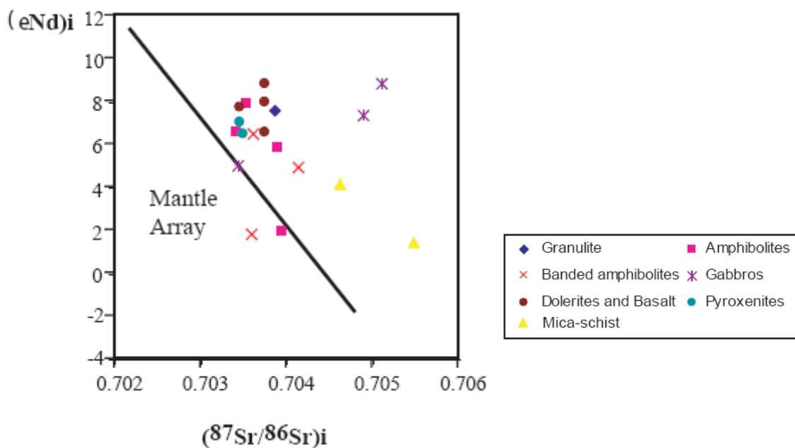
Figure 3.36a. \epsilon Ndi versus (^{87}Sr/^{86}Sr)_i for igneous, metamorphic and ultramafic rocks of Ecuador.
