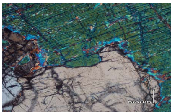
Figure 3.27b. Cumulated pyroxenites : 03SJ4. Opx + cpx + plag. Olivine free. Heterocumulated texture
