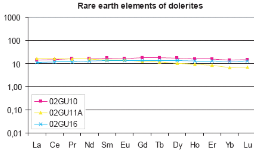
Figure 3.7a. REE of dolerites. Normalized to chondrite (Sun and McDonough, 1989).
