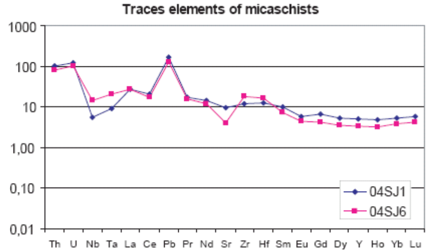
Figure 3.13b. Trace elements of micaschists. Normalized to primitive mantle (Sun and McDonough, 1989).
