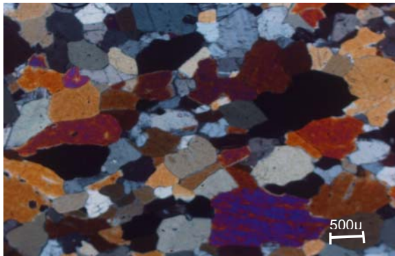
Figure 3.23a. Banded amphibolite : 03GU22B. Plg+amph. Granoblastic texture
