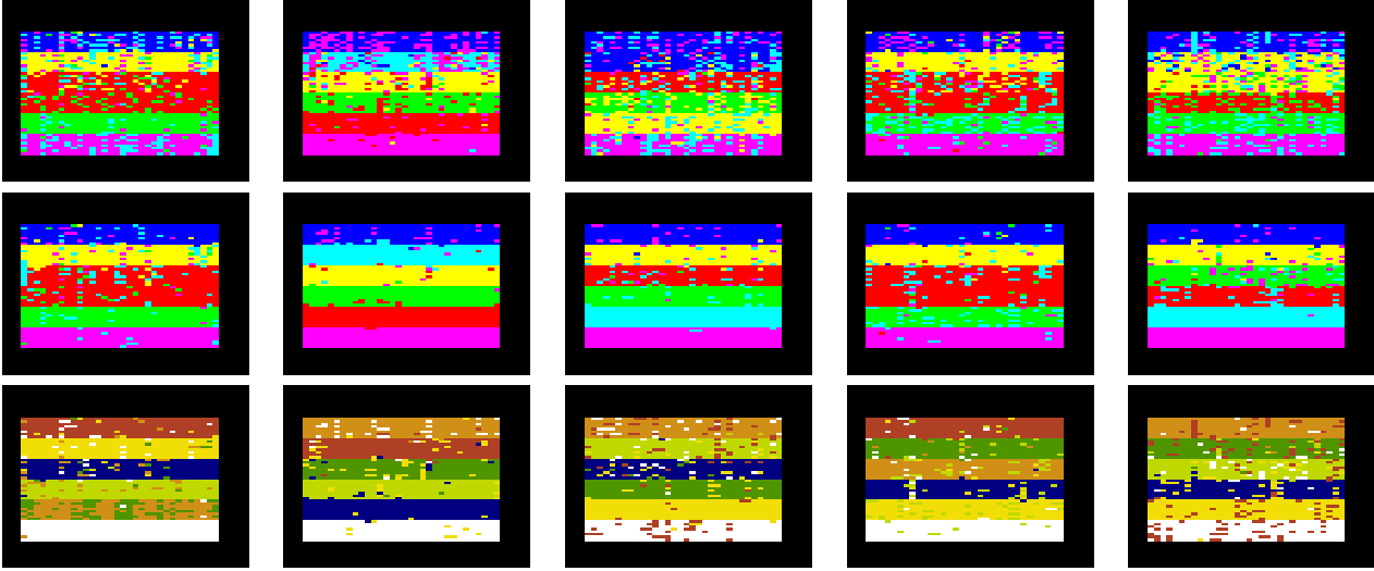
Fig. 3. Top and middle rows: 6 color classifications for 5 synthetic data sets using standard EM algorithm assuming independence (top row) and simulated field algorithm (middle row). Bottom row: 7 color classifications using the Simulated field algorithm. Note that the colors are arbitrarily assigned and may not match.
