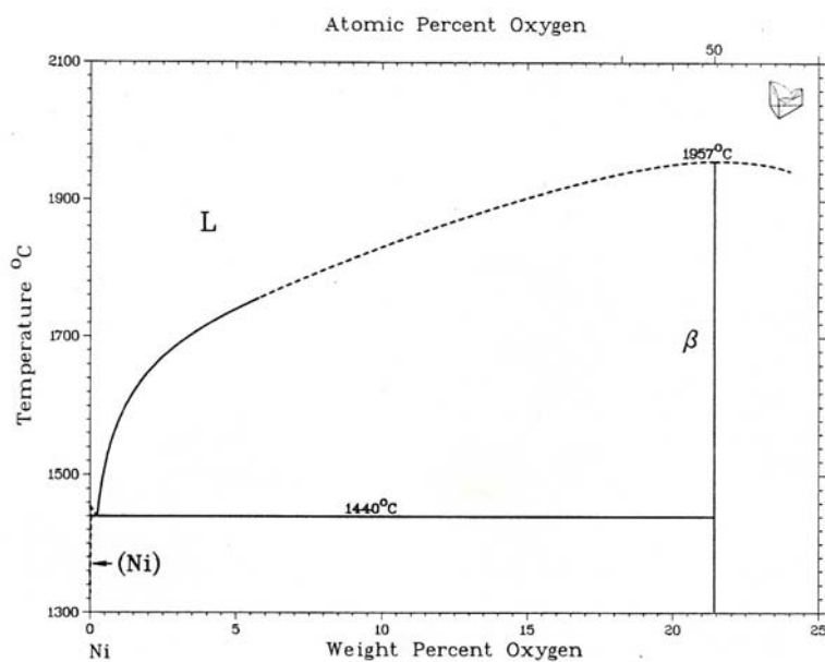
Figure 4-3: The phase diagram of Ni/O.
