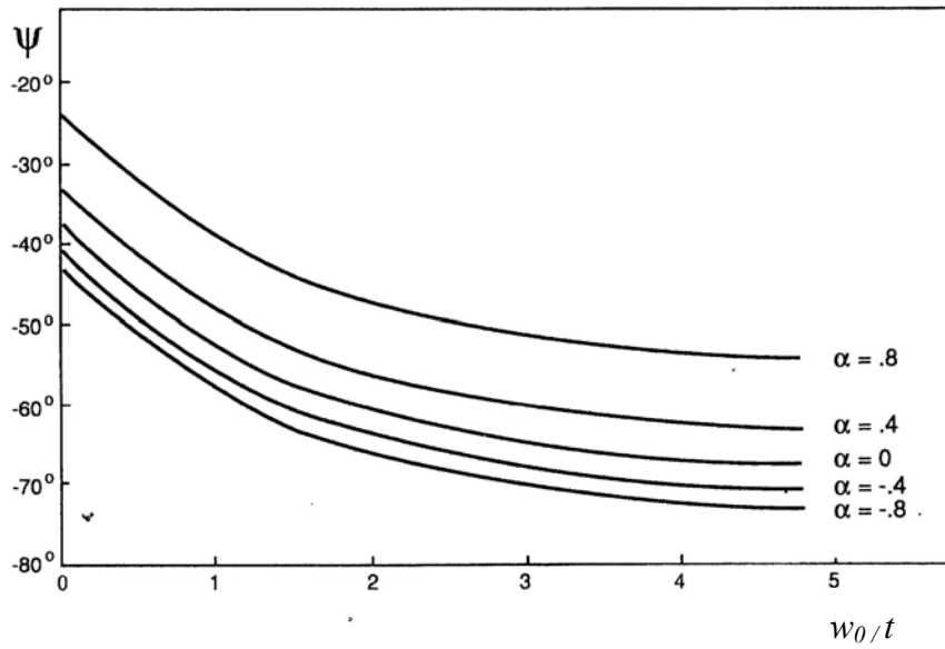
Figure 3-17: the mode mixity of interface crack tip for several levels of elastic mismatch for a blister under a point load [Hutchinson 1992].
