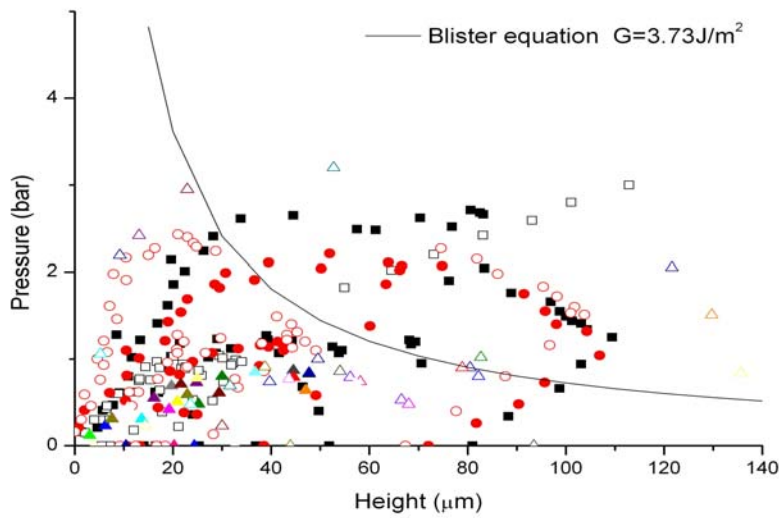
Figure 5-12: The experimental data acquired from blister test and the fitting blister equation, for G_{ci} = 3.73 \text{ J/m}^2 . Ag is fired at 850 °C and BaTiO 3 is fired at 1440 °C. The average surface roughness of BaTiO 3 substrate is 0.21 \mu\text{m} .
