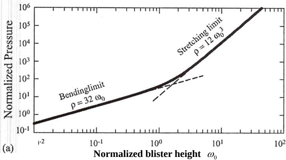
Figure 2-8: The constitutive relation \rho(\omega_0) [Arjun 2005].
