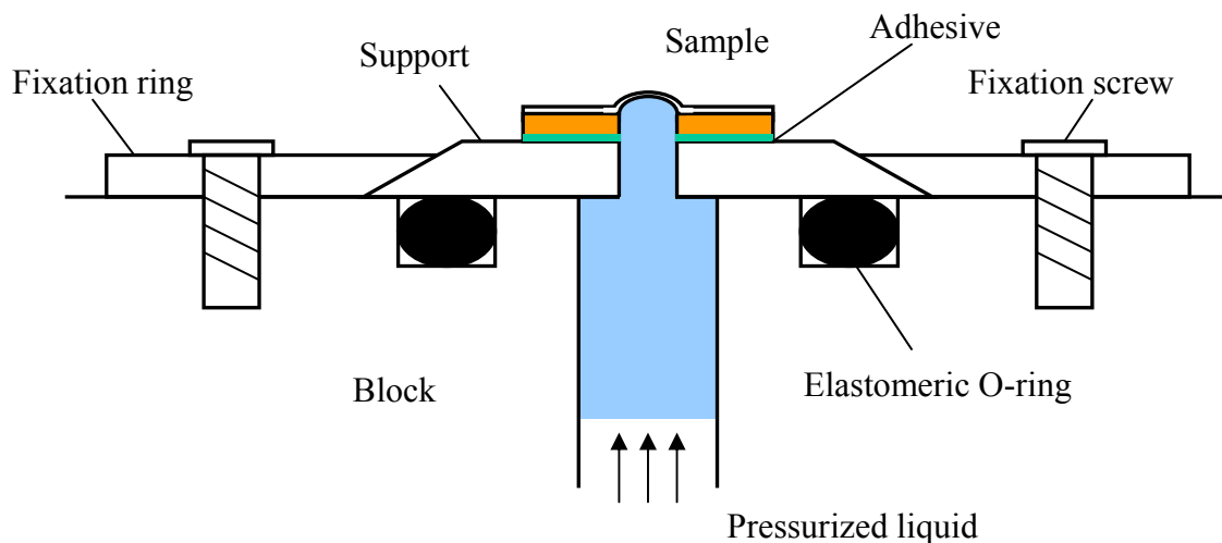
Figure 4-7: Sample mounting
