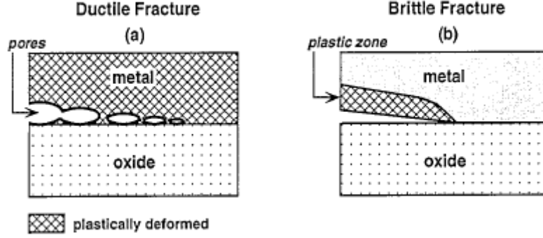
Figure 1-3: Fracture mechanisms for metal-oxide interfaces [Evans 1988, 1993].
