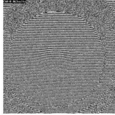
Figure 4-14: Image of calculated phase analyzed by four phase-stepping.
