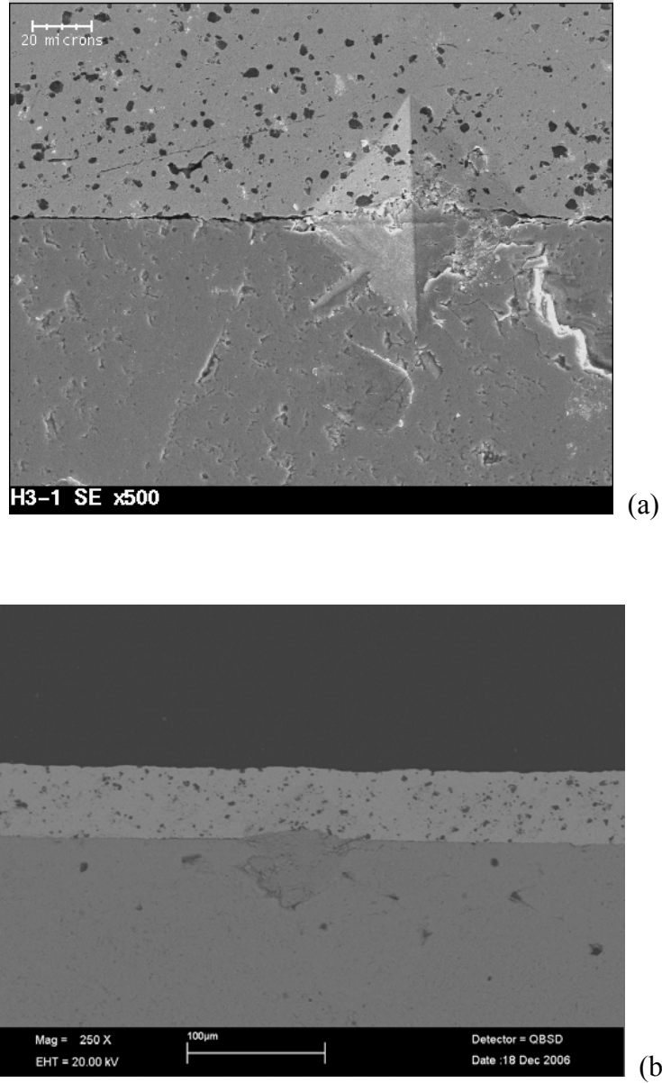
Figure 5-30: Cross-section of Ag/BaTiO 3 interface (a) SE mode (b) BSE mode (scanning electron microscopy).
