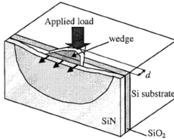
Figure 1-16: Principle of the Cross-sectional nanoindentation test [Sanchez 1999].
