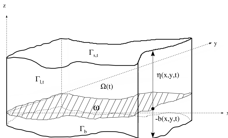
FIG. 6.1 – The three-dimensional domain and its boundaries.
