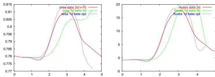
FIG. A.13 – Results of the 1-d model using \beta_{estim} (blue dotted line) and \beta_{3d} (green dashed line), compared to the 3D data (red line), after 70 timesteps.
