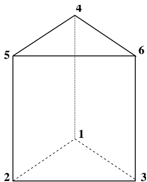
FIG. 6.4 – The first order prismatic element
