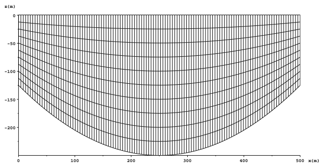
FIG. 4.5 – Vertical cross-section of the initial 3D mesh at y = 50 m.
