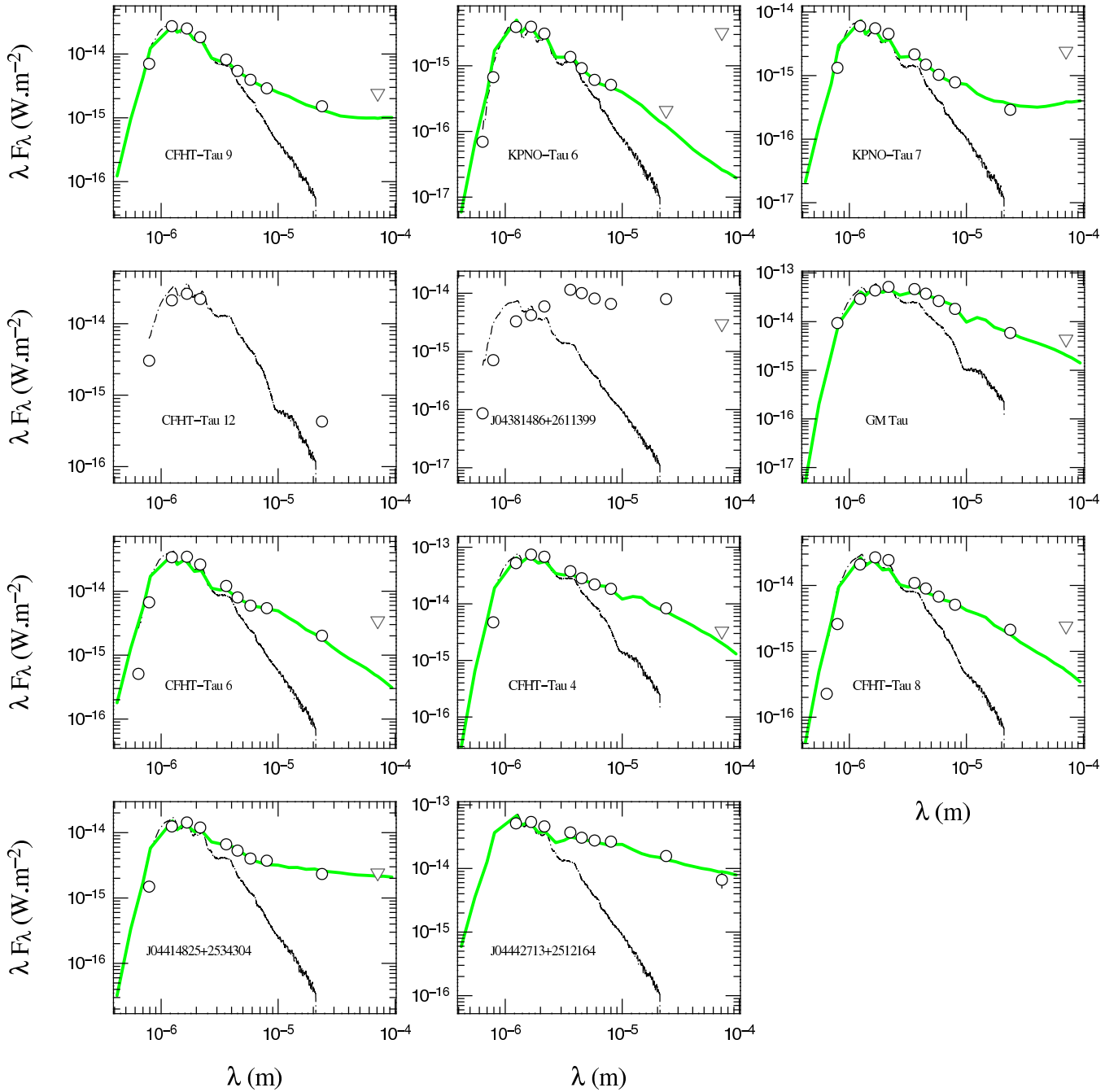
Fig. 2. Same as figure 1 for BDs with infrared excesses. The green line traces our SED models; see text and Section 3 for details.
