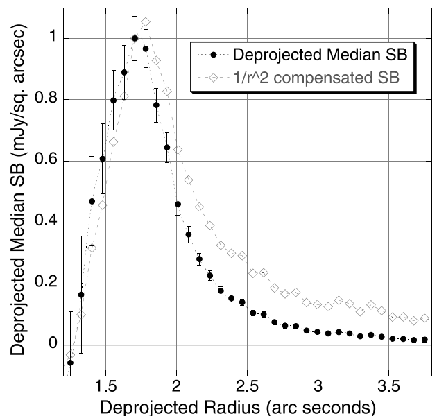
FIG. 7.—Azimuthally medianed 1.1\ \mu\text{m} radial SB profile of the HD 181327 ring (deprojected from an inclination angle of 31.7^\circ from face-on) and the 1\sigma uncertainties in each 75.8 pixel wide annular zone measured. The 1\sigma error bars indicate the dispersion in the NICMOS SB measures around the ring at each elliptical annulus and do not include the \sim 9\% uncertainty in the absolute calibration of the SB. An adjusted profile compensating for the dilution of starlight with distance from the central star normalized to the radius of peak brightness is also shown.
