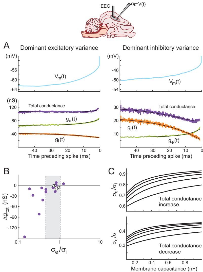
Figure 5.9: Spike-triggered conductance analysis in vivo . A. STA conductance analysis from intracellular recordings in awake and sleeping cats. Two example cells are shown during wakefulness, and for each, the V_m STA (top) and the extracted conductance STAs (bottom) are shown. In the first cell (left), the total conductance increases before the spike. In the second example cell (right), the total conductance decreases before the spike (black traces are exponential fits to the extracted STAs). B. Total conductance change preceding spikes as a function of the ratio \sigma_e/\sigma_i . Given the cell-to-cell variability of observed spike thresholds, each cell has a different predicted ratio separating total conductance increase cases from total conductance decrease cases. The two dashed lines ( \sigma_e/\sigma_i=0.48 and \sigma_e/\sigma_i=1.07 ) visualize the two extreme predicted ratios. Cells in white are the ones not conforming to the prediction. C. Dependency of the ratio \sigma_e/\sigma_i estimated by the VmD method on the value of the membrane capacitance C . Two sets of realistic V_m distribution parameters were used as input for the estimation, one leading to \sigma_e/\sigma_i > 0.6 (left), another leading to \sigma_e/\sigma_i < 0.6 (right). For each set, the total input resistance was varied from 10 M \Omega (bottom curves) to 50 M \Omega (top curves), in steps of 10 M \Omega . Panel A modified from Rudolph et al., 2007.
