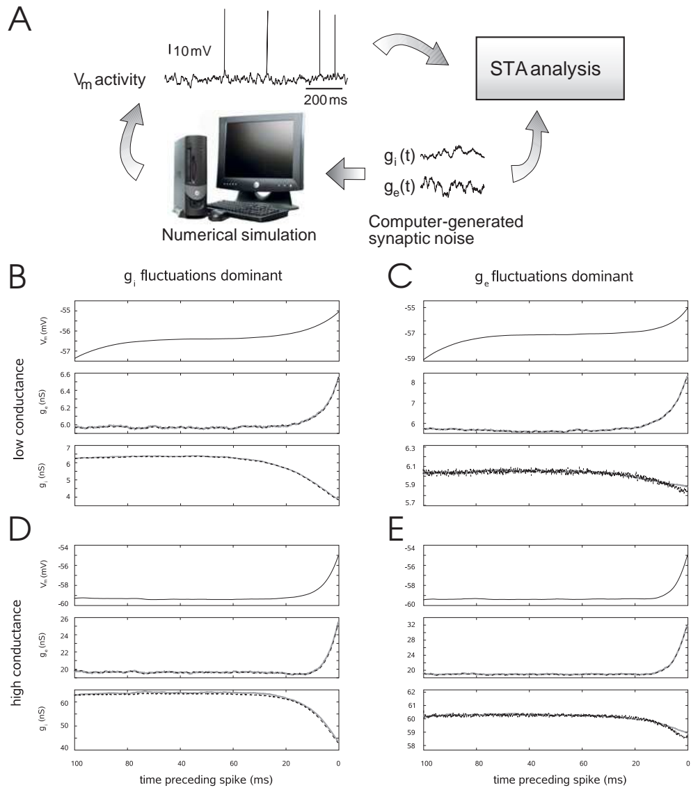
Figure 3.1: Test of the STA analysis method using an IF neuron model subject to colored conductance noise. A. Scheme of the procedure used. An IF model with synaptic noise was simulated numerically (bottom) and the procedure to estimate STA was applied to the V_m activity (top). The estimated conductance STAs from V_m were then compared to the actual conductance STA in this model. Bottom panels: STA analysis for different conditions, low-conductance states (B,C), high-conductance states (D,E), with fluctuations dominated by inhibition (B,D) or by excitation (C,E). For each panel, the upper graph shows the voltage STA, the middle graph the STA of excitatory conductance, and the lower graph the STA of inhibitory conductance. Solid lines (grey) show the average conductance recorded from the simulation, while the dashed line (black) represents the conductance estimated from the V_m . Parameters in B: g_{e0}=6 nS, g_{i0}=6 nS, \sigma_e=0.5 nS, \sigma_i=1.5 nS; C: g_{e0}=6 nS, g_{i0}=6 nS, \sigma_e=1.5 nS, \sigma_i=0.5 nS; D: g_{e0}=20 nS, g_{i0}=60 nS, \sigma_e=4 nS, \sigma_i=12 nS; E: g_{e0}=20 nS, g_{i0}=60 nS, \sigma_e=6 nS, \sigma_i=3 nS
