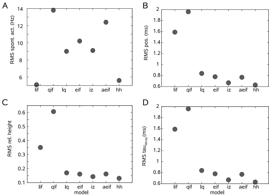
Figure 6.5: Comparison of different characteristics of the PSTH. The RMS error of the difference between the experimental and the model PSTHs are given. A : spontaneous activity. B : PSTH peak position. C : relative peak height. D : PSTH decay time constant. With exception of spontaneous activity, the model performance followed the ranking of Fig. 6.4.
