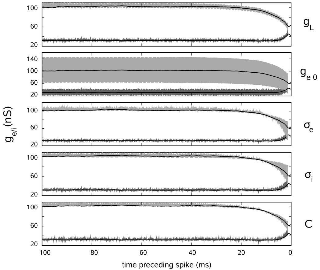
Figure 3.6: Deviation in the estimated conductance STAs in real neurons using dynamic-clamp due to variations in the parameters. The black lines represent the conductance STA estimates using the correct parameters, the gray areas are bound by the estimates that result from variation of a single parameter (indicated on the right) by \pm 50\% . Light gray areas represent inhibition, dark gray areas represent excitation. The total conductance (leak plus synaptic conductances) was assumed to be fixed. A variation in the mean values of the conductances evokes mostly a shift in the estimate, while a variation in the SDs influences the curvature just before the spike.
