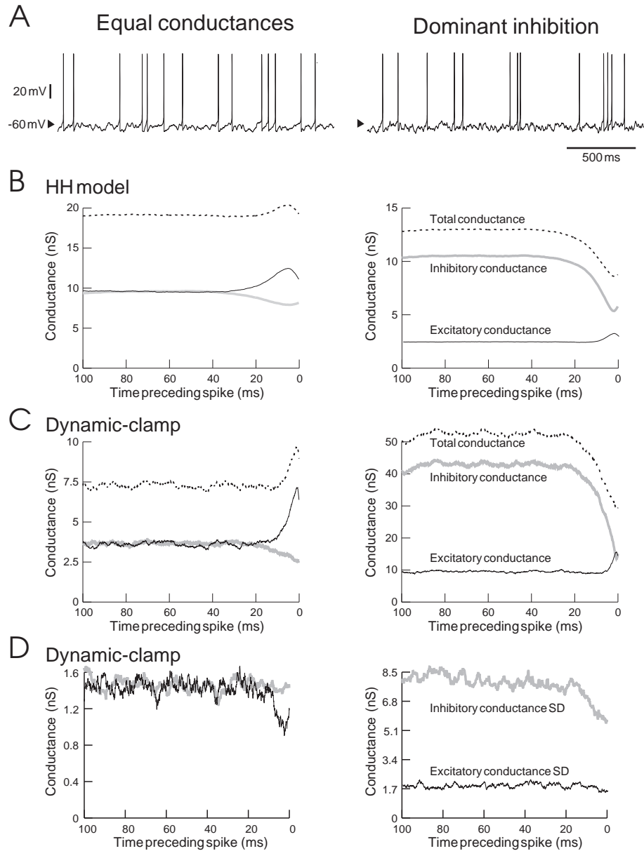
Figure 2.1: Optimal patterns of conductance related to spikes in cortical neurons. Comparison of low-conductance (left) and high-conductance states (right). A spike is evoked at t = 0 ms. A . The voltage traces in the two states obtained in models are similar in terms of V_m mean and variance (model). B . Spike-triggered average of inhibitory, excitatory and total conductance in the model. In the LC state, the spike is preceded by a peak in excitatory and total conductance, whereas in the HC state there is a marked drop of inhibitory and total conductance just before the spike. C . Same as B for guinea-pig cortical neurons under dynamic-clamp. D . Conductance standard deviations (SD) from the same experiment as in C : in the LC state, only excitatory SD drops before the spike, whereas in the HC state only inhibitory SD shows a significant decrease.
