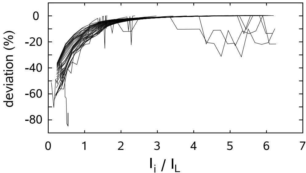
Figure A.2: Relative deviation between the parameter \sigma_i in the simulations and its re-estimated value depending on the ratio of the currents due to inhibitory and leak conductance. The estimation fails, when the inhibitory component becomes too small.
