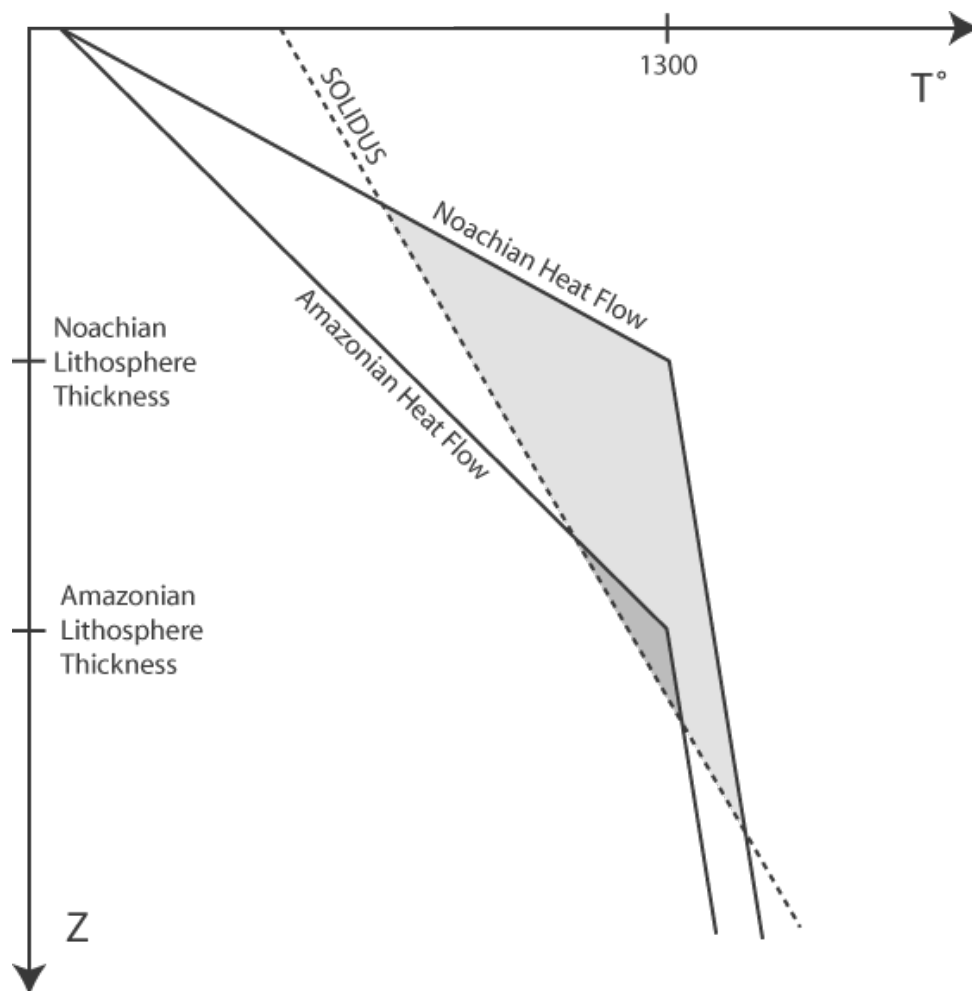
FIG. 9.10 – Illustration of the possible origin of lower partial melting under thick lithosphere. The lithosphere, which base is the 1300^\circ\text{C} thermal boundary, is supposed thinner during Noachian period than during Amazonian period, yielding to greater partial melting during the Noachian (light grey) than during the Amazonian (dark grey). Thus it is likely that the current martian volcanism results from low partial melting considering the current martian lithosphere thickness.
