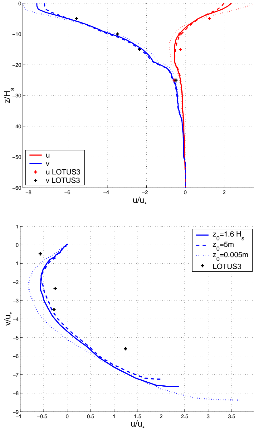
Figure 3.8: Results of the LOTUS 3 simulation, without the Stokes-Coriolis force, with the observed wind stress and with the temperature constrained to the data. (Upper panel) Vertical profiles of the mean current \hat{u} , \hat{v} . (Lower panel) Spirals of the mean current. Solid lines are the default model ( z_0 = 1.6H_s^{FD} ), dashed line are the model with a large surface mixing ( z_0 = 5\text{ m} ), and dotted lines, without the wave-induced mixing ( z_0 = 0.005\text{ m} ).
