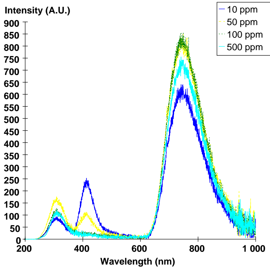
Figure 4.18: Scintillation spectra of \text{Ti}:\text{Al}_2\text{O}_3 crystals with a Ti concentration of 10, 50, 100 and 500 ppm at 45 K.
