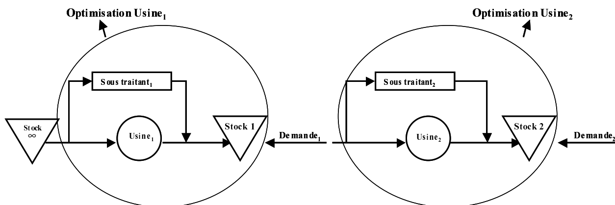
Fig. 2.8 – Optimisation Locale (OL)
