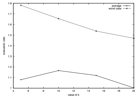
Fig. 12. Heuristic on weights. Simulation with large weights.
