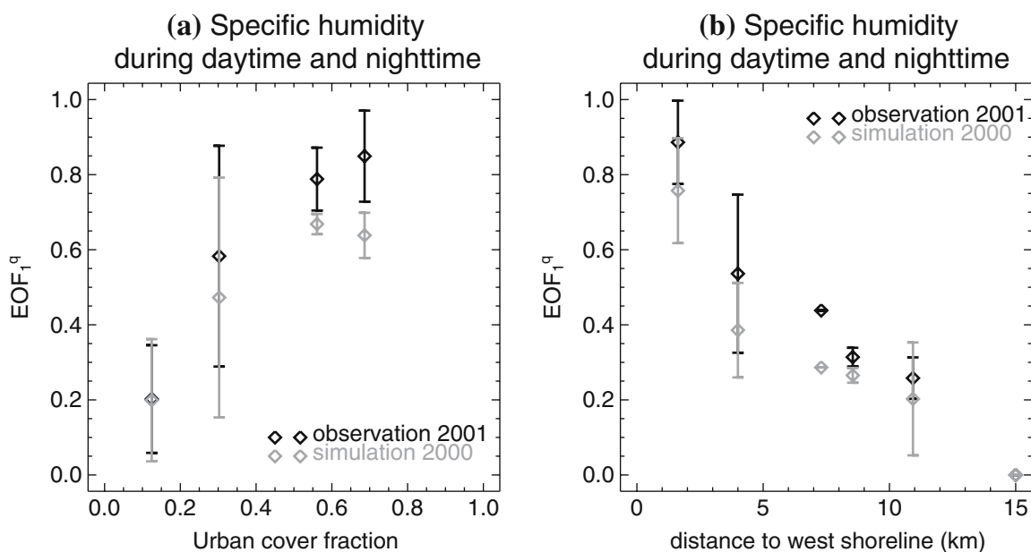
Figure 20. Same as Figure 19 but for q during daytime and nighttime.
