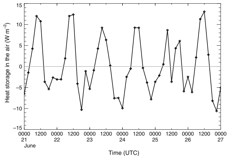
Fig. 5 Heat storage in the air during IOP2a and IOP2b computed with the tower air temperature profile and an estimate of the air temperature at z_H (three-hourly averages reported)
