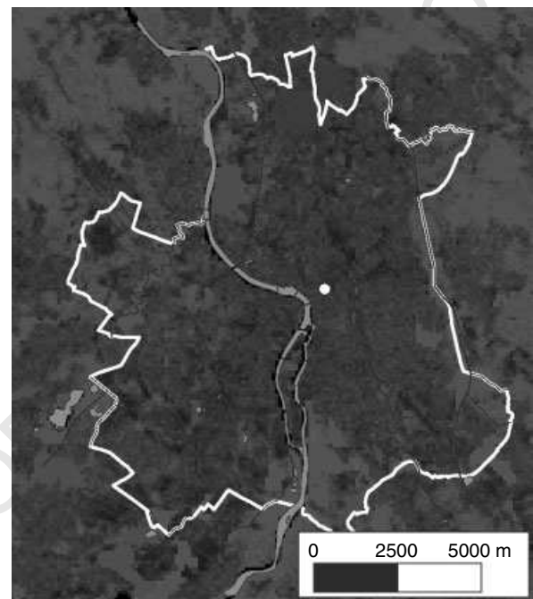
91 Figure 1. Colour composite of building plan area density (pad, in red), 92 vegetation pad (in green) and road pad (in blue) with 100-m resolution 93 over the agglomeration of Toulouse. The white line represents the 94 limit of Toulouse district. This figure is available in colour online at www.interscience.wiley.com/ijoc
