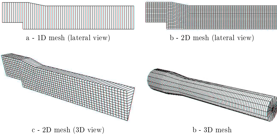
FIG. E.2 – Examples of meshes
