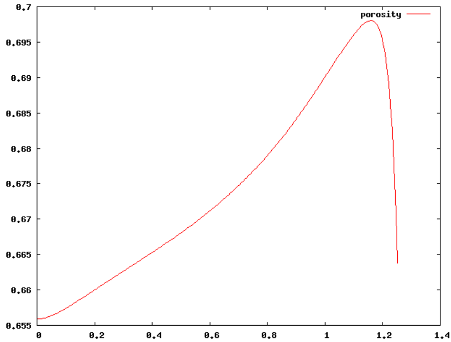
FIG. 4.15 – Porosity at the final time. Relaxation model with granular stress.
