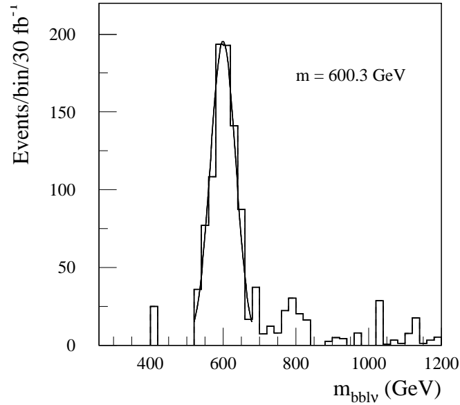
Fig. 5 - The background subtracted mass distribution fitted with a Gaussian in case of an exchanged \bar{s} -quark of 600 GeV for a ub initial parton state. It corresponds to 3 years of LHC run with low luminosity.
