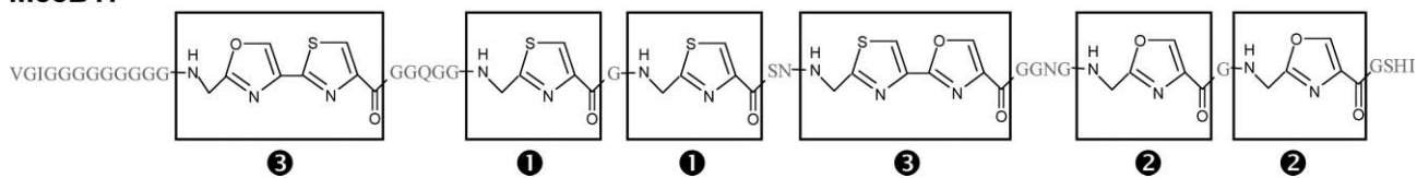
Fig. 2 Sequence of the Mccb17 precursor (McbA) and structure of mature Mccb17. The 26-residue leader peptide is underlined in McbA. The amino acids are figured in grey for mature Mccb17. In Mccb17, thiazoles (1), oxazoles (2), and bis-heterocycles (3) are boxed.
