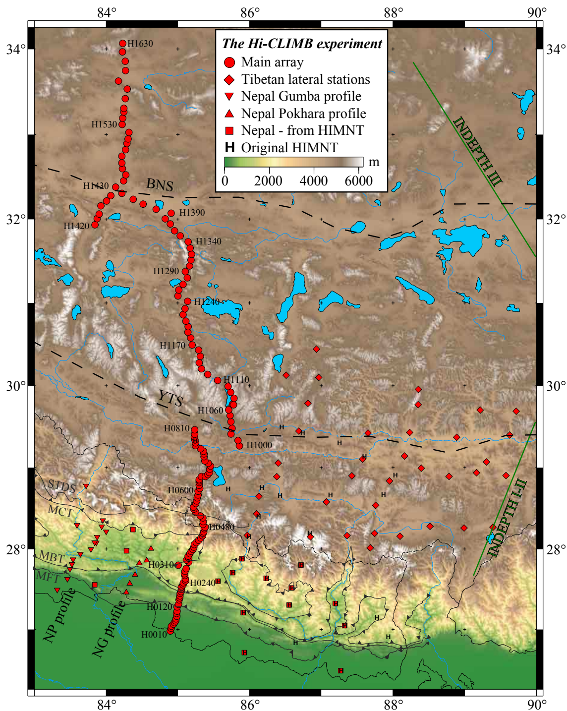
Figure 3.1: Stations of the Hi-CLIMB experiment. Red symbols mark the different groups of Hi-CLIMB stations, also summarized in Table 3.1. For better readability, only a few stations are identified along the main array. Complete station information is available in Appendix B. HIMNT station locations are noted for reference. HIMNT is "Himalayan Nepal Tibet earthquake seismic experiment" (see e.g. Schulte-Pelkum et al., 2005). Major sutures (YTS: Yarlung Tsangpo Suture, BNS: Banggong-Nujiang Suture) and faults, as well as the approximate lines of the INDEPTH experiments are drawn for reference.
