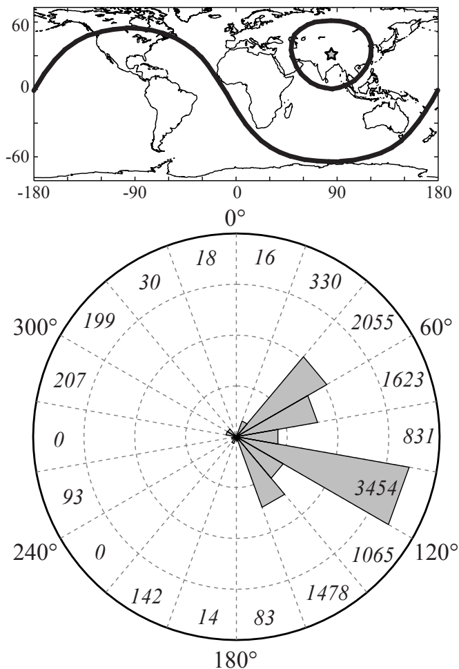
Figure 3.13: Top: iso-epicentral distance lines at 30 and 95° from the centre of the Hi-CLIMB main array (star). Earthquakes within this range are suitable to produce RFs. Bottom: back-azimuthal statistics of a selection of traces used for migration along the main profile (W3 list after second quality control).
