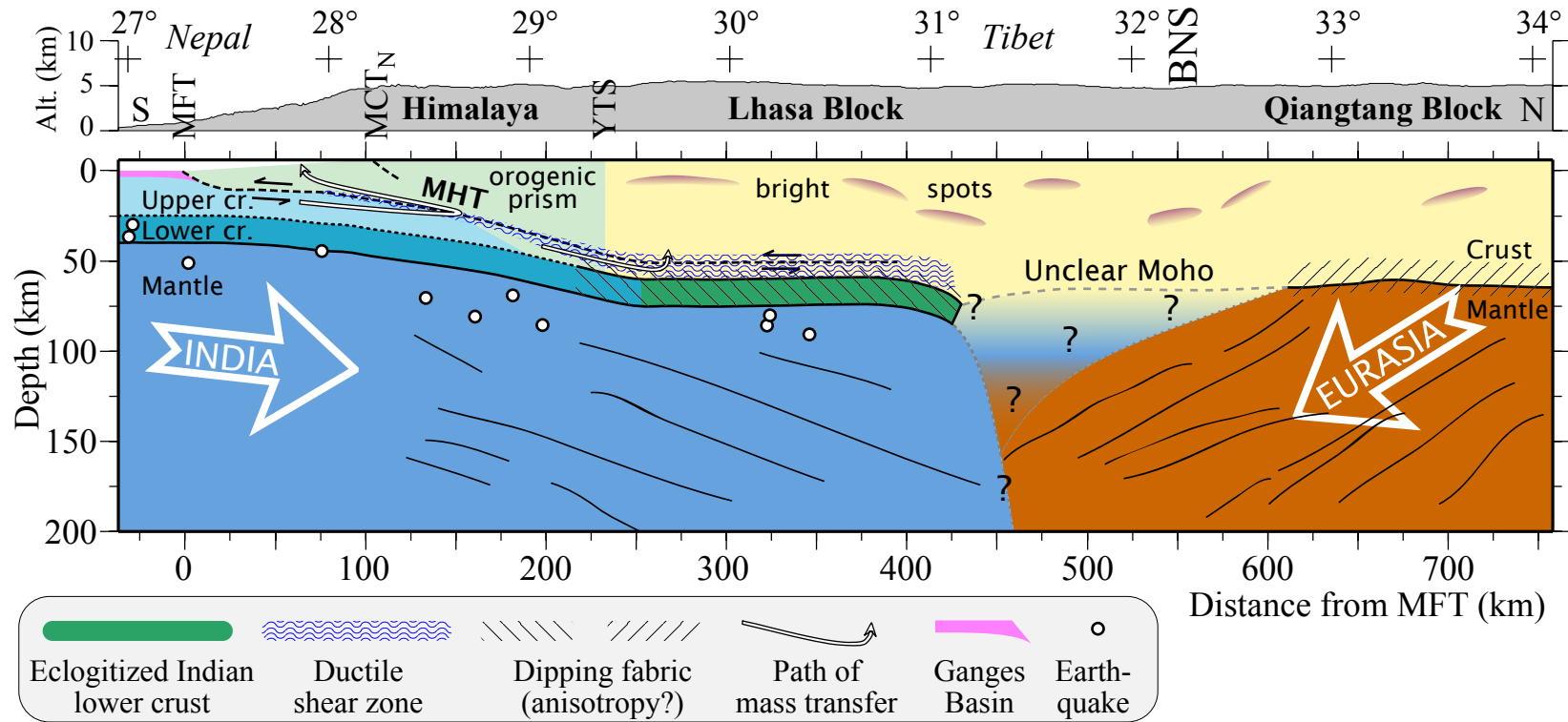
Figure 5.17: Interpretative scheme of the India-Eurasia collision zone as seen by the Hi-CLIMB experiment. The Indian lithosphere underplates the Tibetan Plateau on ~450 km, including its lower crust which undergoes eclogitization. The Main Himalayan Thrust (MHT), already ductile beneath the Himalayas, merges to a mid-crustal low-velocity zone in Lhasa block and accommodates the convergence. It also allows upper crustal material to build the Himalayas as well as Lhasa block by crustal thickening from below. The Moho beneath Qiangtang block is ~10 km shallower than beneath Lhasa block. Upper crustal bright spots are observed in both southern and northern Tibet. The polarity of both the Moho and the lower lithosphere reflects the different tectonic origin and evolution of the Indian and Eurasian lithospheric blocks. The main boundary between them is located south of the BNS and is marked with an unclear crust-mantle boundary. Earthquakes (from Chen and Yang, 2004) suggest currently active deformation within the uppermost mantle. MFT: Main Frontal Thrust. MCT N : northern expression of the Main Central Thrust.
