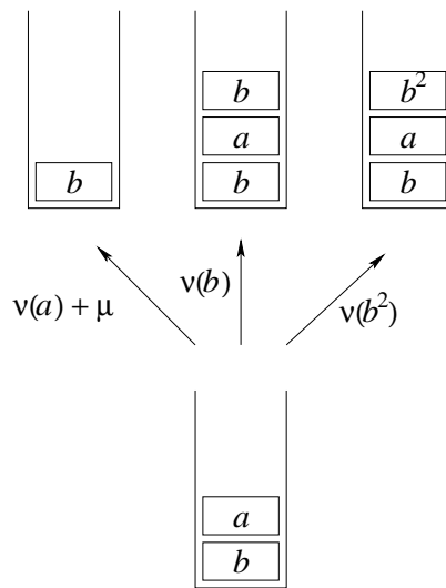
FIGURE 7.1 – The queue-content’s evolution of the LIFO queue associated to \mathbb{Z}/2\mathbb{Z} \star \mathbb{Z}/3\mathbb{Z}
