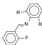
30a R = Me 30b R = i -Pr
