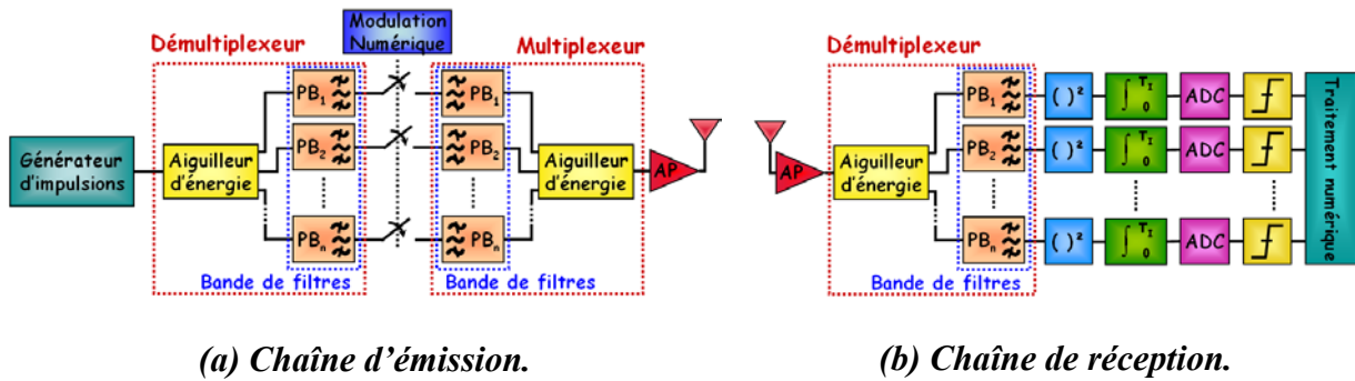
Figure III.13 : Système de transmission MB-OOK.
