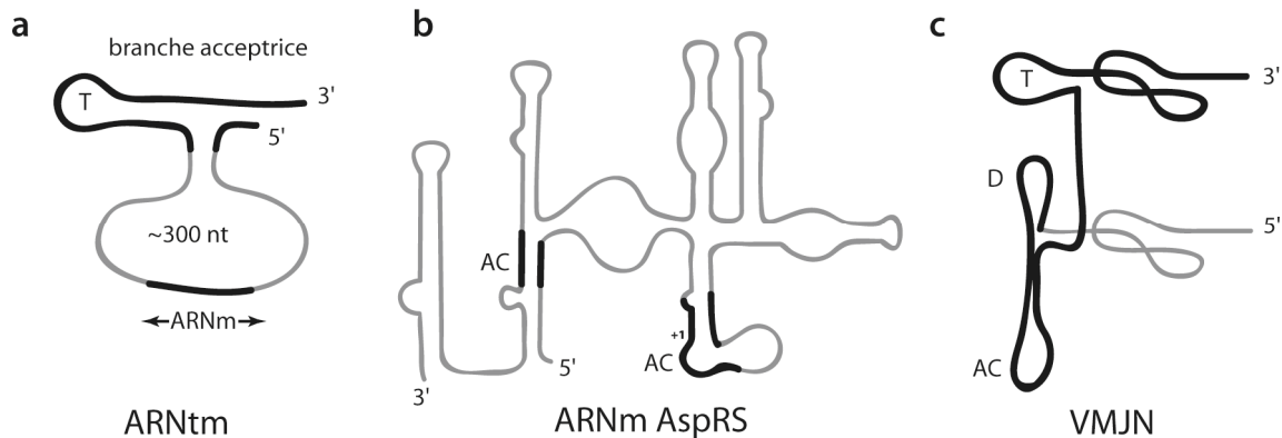
Figure 2. Structures pseudo-ARNt
