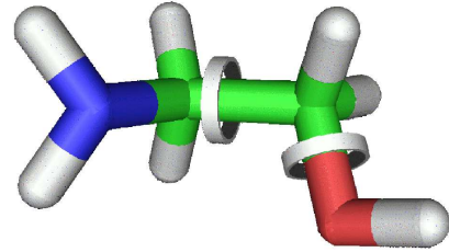
Fig. 1. Torsional angle coding.
