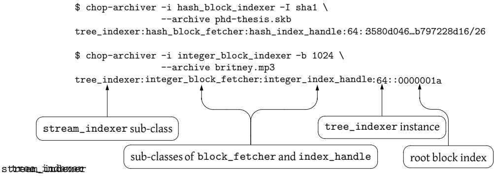
Figure 43. ASCII-serialized index produced by libchop 's storage process.
