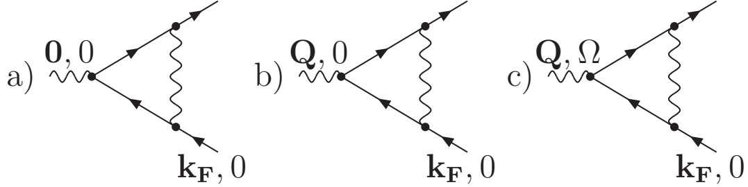
Figure 2.2: Three-leg vertices: a) zero external momentum and frequency b) finite momentum c) generic vertex.
