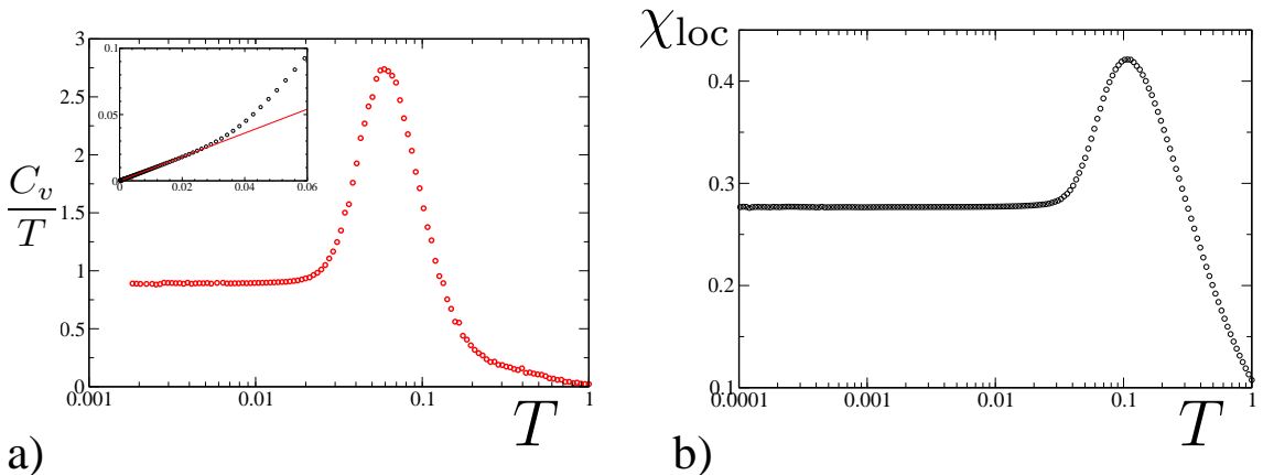
Figure 6.12: ES case: a) Specific heat coefficient for \gamma = 0.1 as a function of temperature on a log scale. Inset: the low temperature entropy shows a linear behavior. b) Temperature variation of the local spin susceptibility for \gamma = 0.1 . The saturation of both quantities is consistent with a Fermi liquid behavior.
