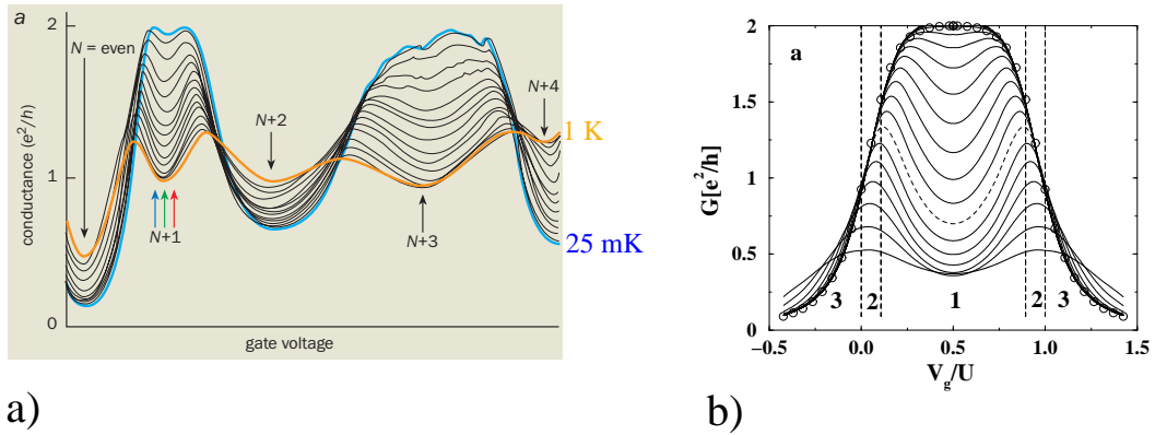
Figure 5.5: a) Experimental observation of the effect of the Kondo resonance on the conductance of a dot [82]; b) These lineshapes could be recovered theoretically using a numerical renormalization group approach [83].
