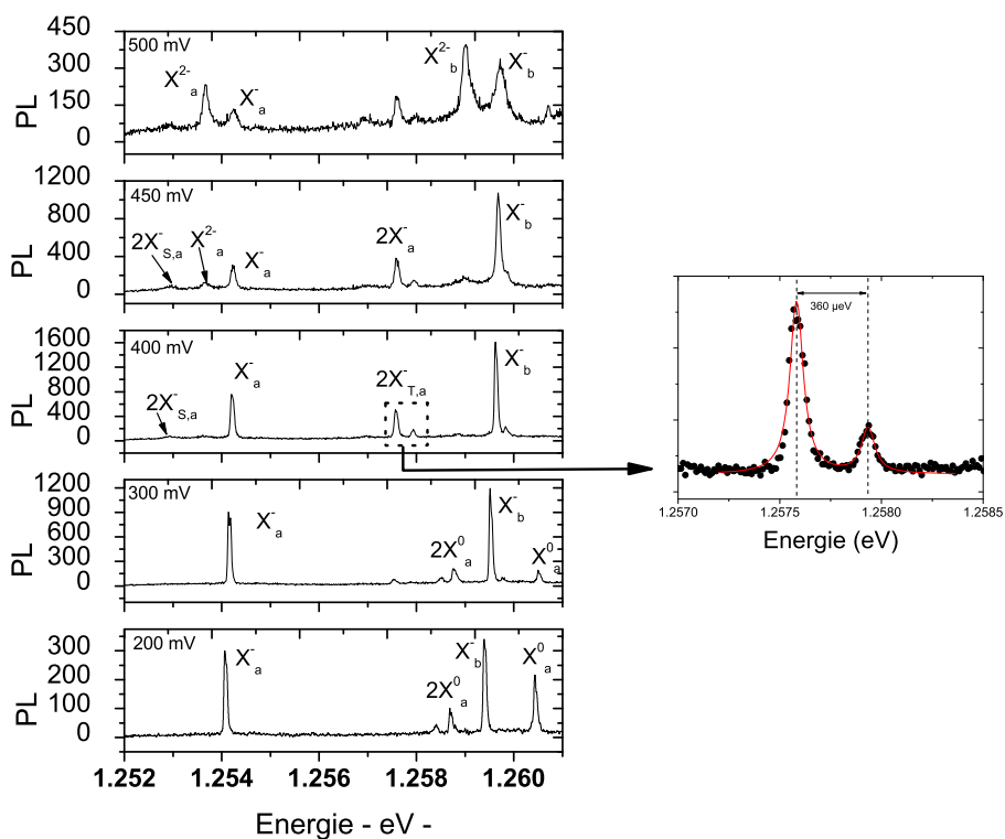
FIG. 2.22: Observation de 2X^-
