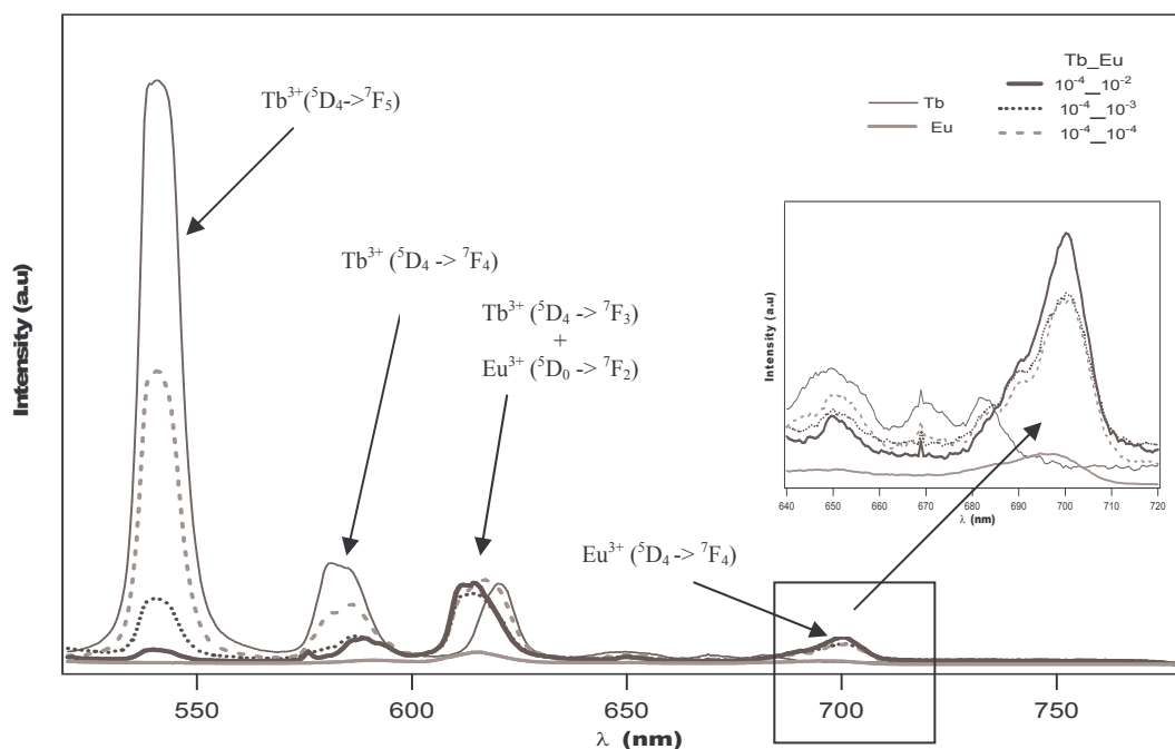
Fig. 4: Luminescence spectra at 25°C (at an excitation wavelength of 487 nm) for only Tb^{3+} sorbed onto SrTiO_3 , for only Eu^{3+} sorbed onto SrTiO_3 and for Tb^{3+}/Eu^{3+} sorbed onto SrTiO_3 .
