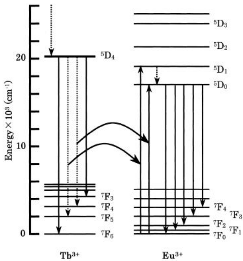
Fig. 2: Energy level diagrams of Tb^{3+} and Eu^{3+} ions (from reference [22]).
