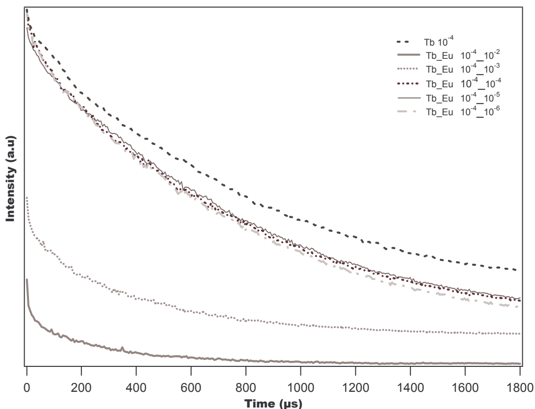
Fig. 5: Logarithmic plot of the fluorescence decay of Tb^{3+} ions at room temperature for different systems: for SrTiO_3 only sorbed with Tb^{3+} and for SrTiO_3 sorbed with Tb^{3+} 10^{-4} M / Eu^{3+} mixtures ( [Eu^{3+}] from 10^{-6} M to 10^{-2} M ) by monitoring the emission line {}^5D_4 \rightarrow {}^7F_5 of Tb^{3+} at 544 nm.
