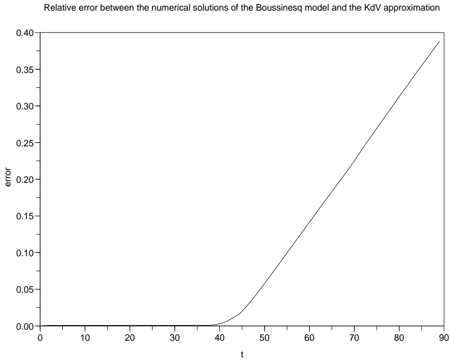
Figure 6.2.2: Relative L^\infty error between the free surfaces for \varepsilon = 0.05
