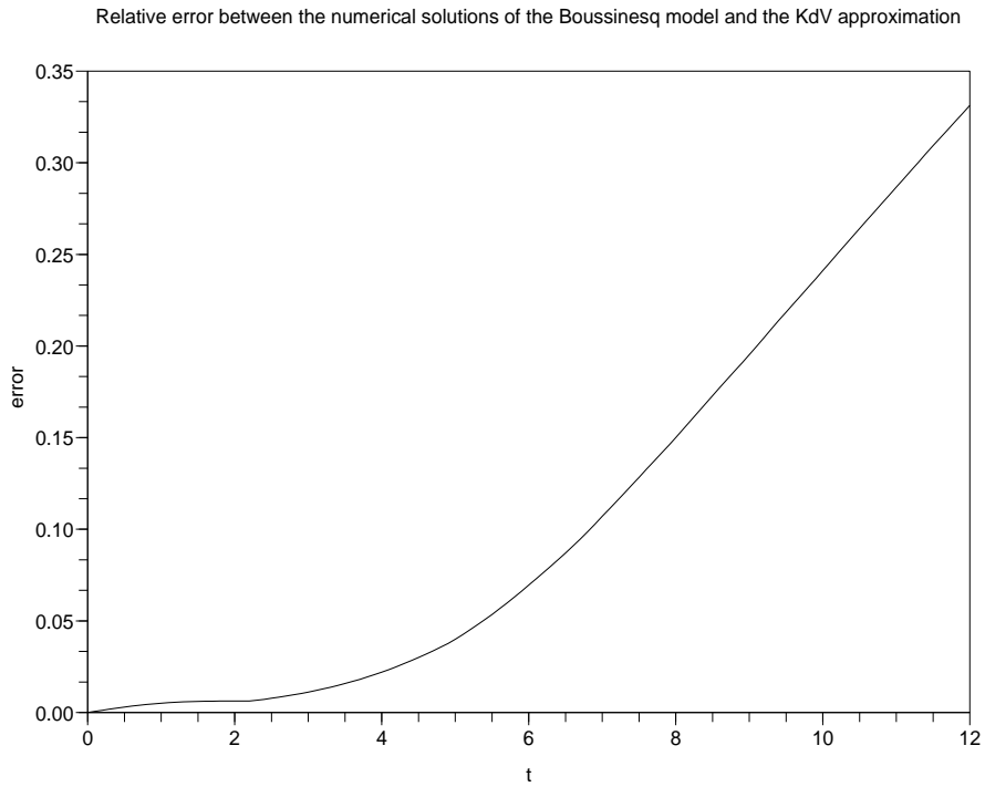
Figure 6.2.6: Relative L^\infty error between the free surfaces for \varepsilon = 0.2
