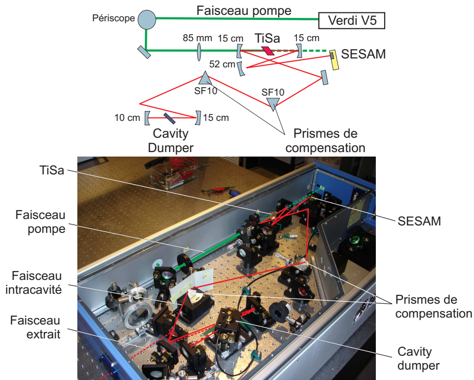
Figure 3.1: Laser impulsif Tiger CD.
