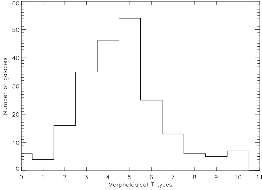
Figure 6.2: Morphologies.
