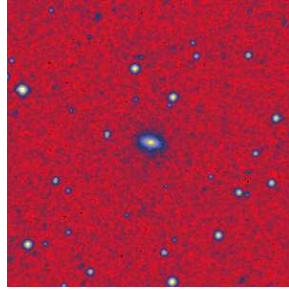
Figure 3.11: CIG 0233.
