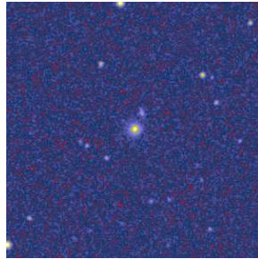
Figure 3.14: CIG 0533.
