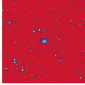
Figure 3.8: CIG 0036.
