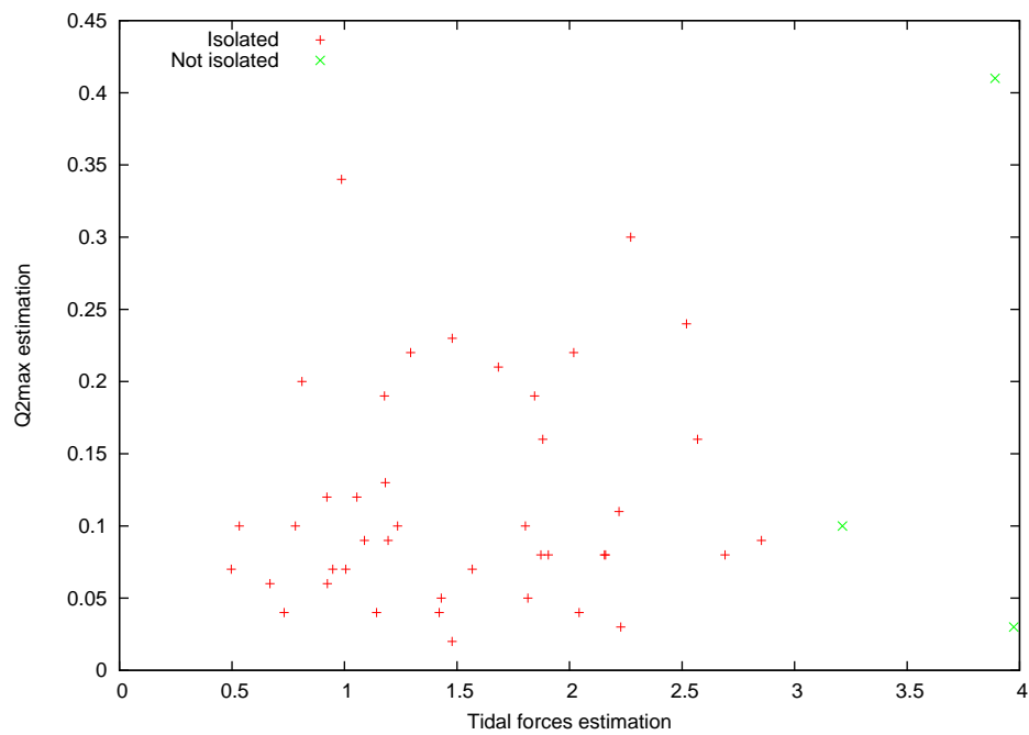
Figure 8.48: Q_2\text{max} .
