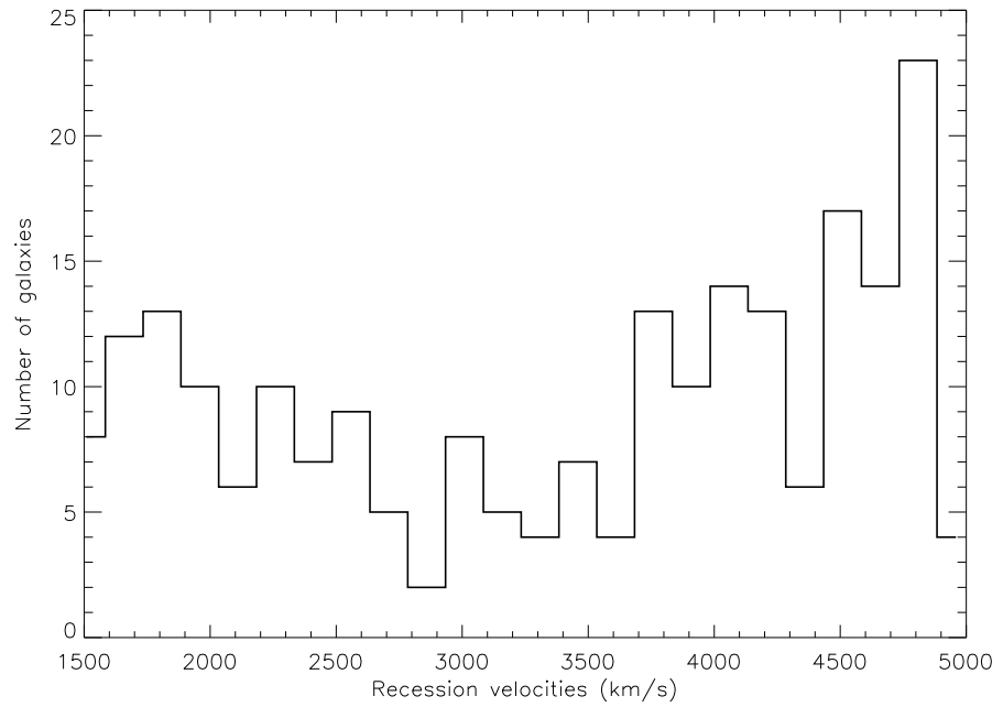
Figure 6.4: Recession velocities.
