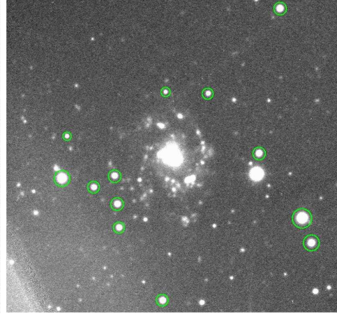
Figure 7.2: Raw H\alpha image.
