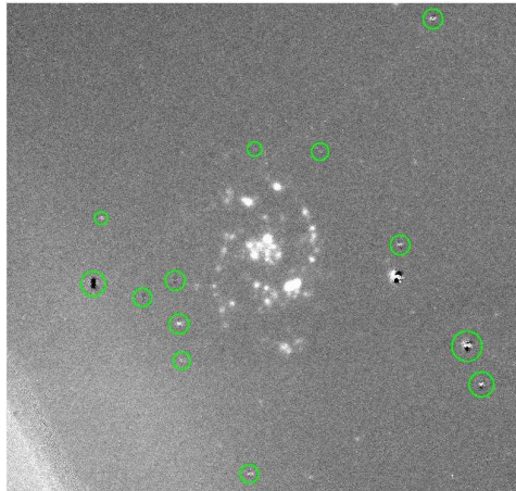
Figure 7.4: H\alpha - continuum.
