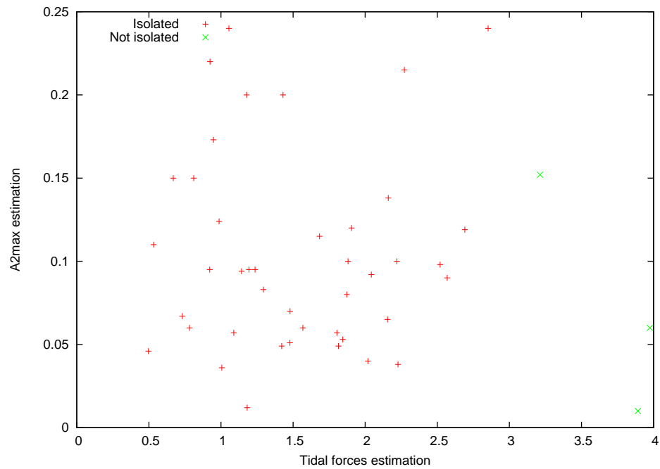
Figure 8.50: A_2\text{max} .
