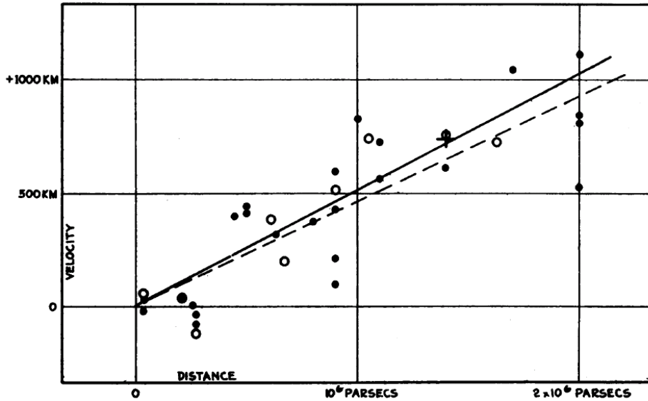
Figure 1.1: Hubble's velocity-distance relation.
