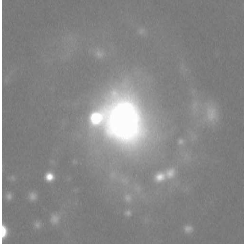
Figure 7.5: r Gunn with stars.
