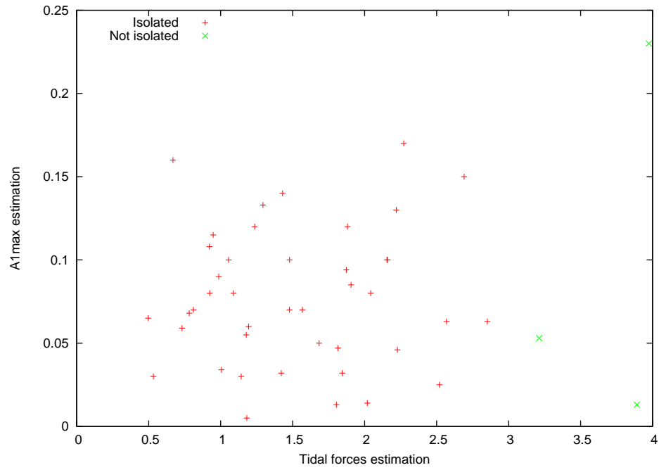
Figure 8.49: A_1\text{max} .
