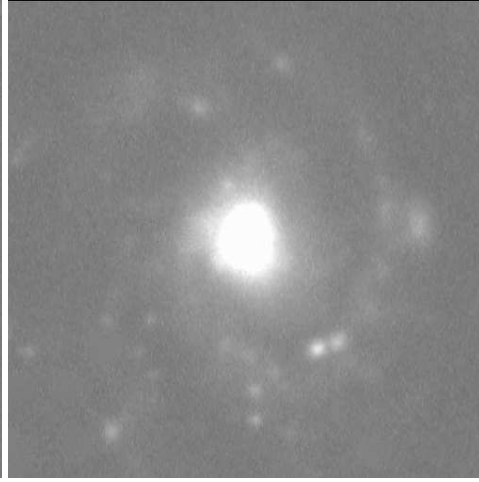
Figure 7.6: r Gunn without stars.
