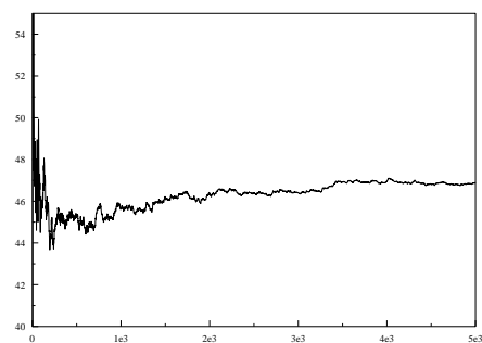
Figure 3.11: Standard Monte Carlo
