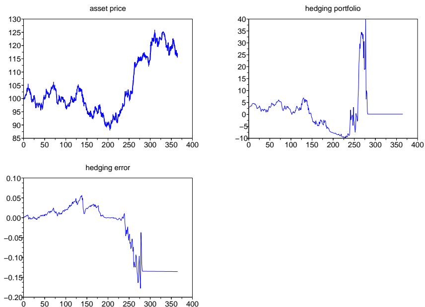
Figure 4.4: Example of delta hedging of a PUOC S_0 = 100 K = 100 T = 1 L = 110 D = 20 day \sigma = 0.2 r = 0.025 \delta = 0
