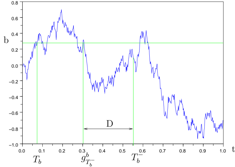
Figure 4.1: Excursion of Brownian Motion
