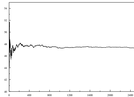
Figure 3.14: Averaging Importance Sampling with MC
