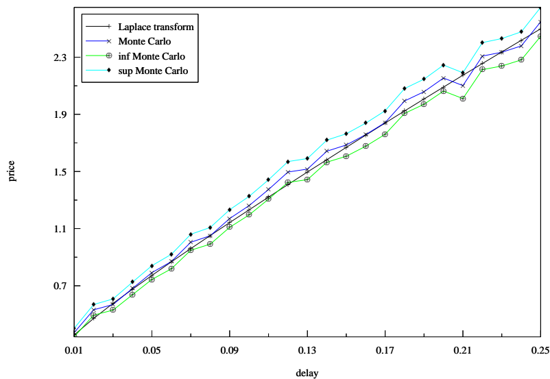
Figure 4.5: Comparison with improved Monte Carlo method in the case of a PDOP S_0 = 100 K = 100 T = 1 L = 90 \sigma = 0.2 r = 0.025 \delta = 0
