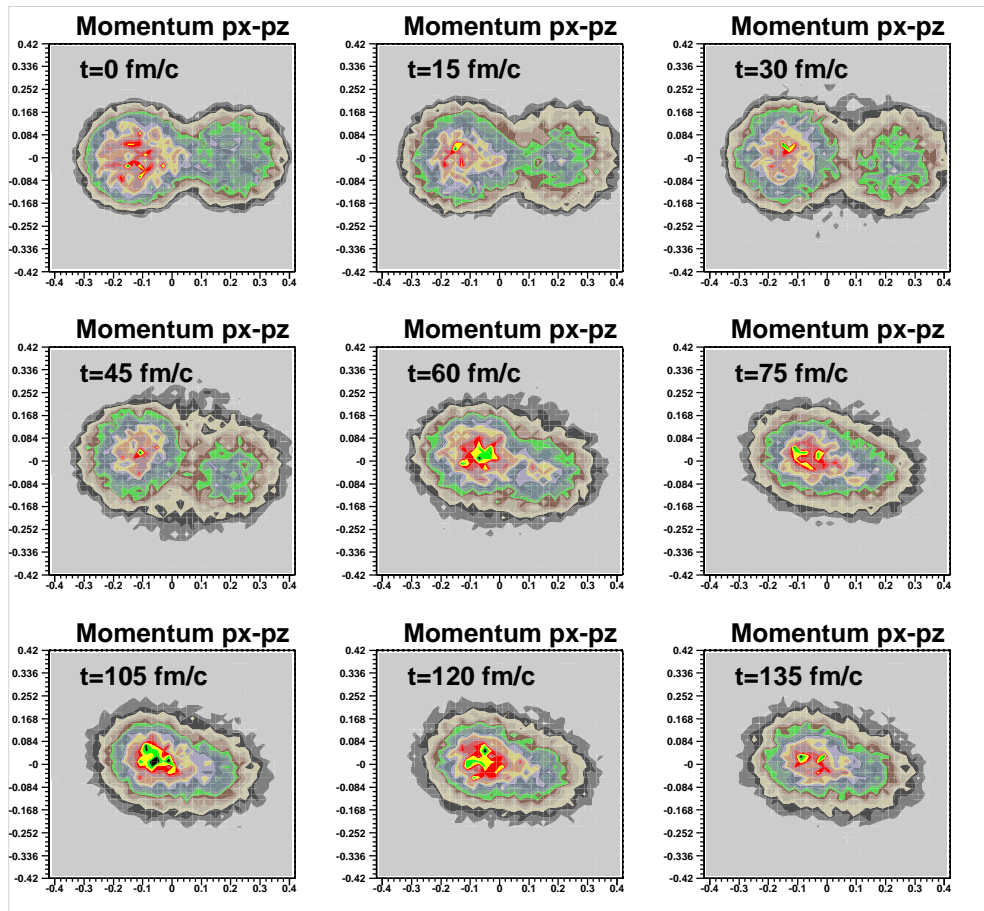
Figure 8.19: Time evolution according to QMD of the reaction ^{36}\text{Ar}+^{58}\text{Ni} at 60A MeV ( b = 2.5 fm), shown as the density distribution of nucleons projected in the transverse-longitudinal ( p_x, p_z ) momentum space. (The units in both axes are GeV/c).
