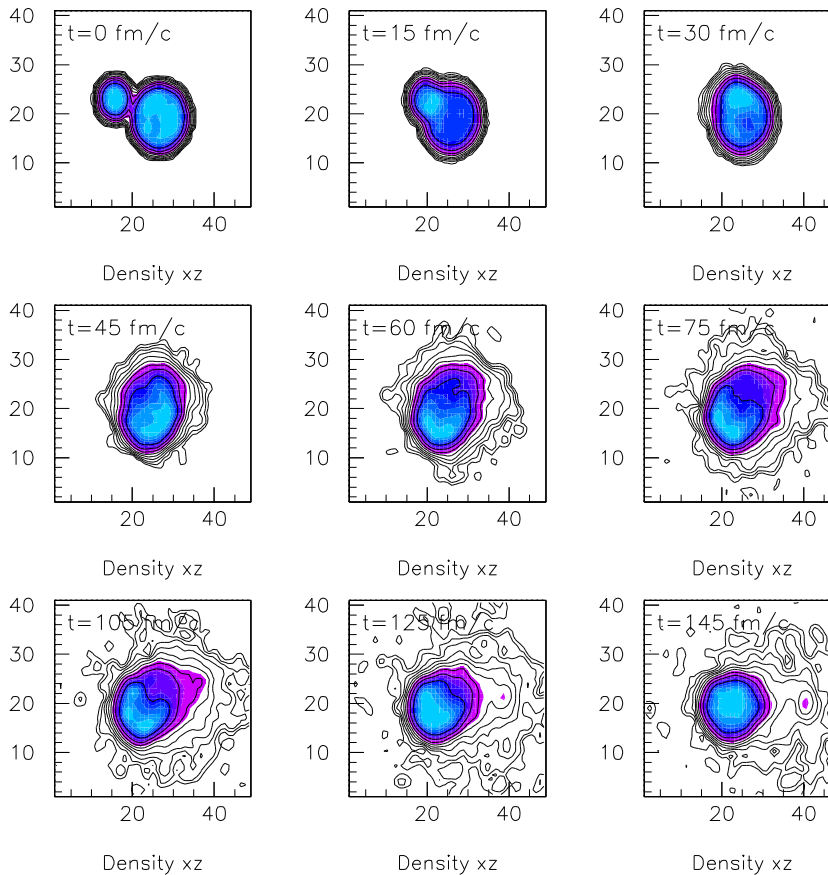
Figure 8.1: Time evolution according to BUU of the reaction ^{36}\text{Ar}+^{197}\text{Au} at 60A MeV and b = 3.8 fm, shown as the density distribution of nucleons projected in the x, z coordinate space. The beam axis is along z , and (x, z) are measured in fm.
