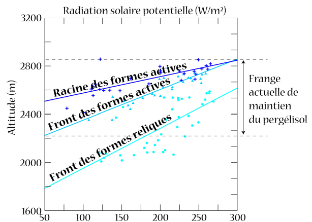
Figure IX-8 : Relation entre la radiation solaire et l'altitude des formes fluantes actives et des formes reliques du massif du Combeynot. Relationship between potential solar radiation and elevation of the active and relict creeping landforms on the Combeynot Massif.
