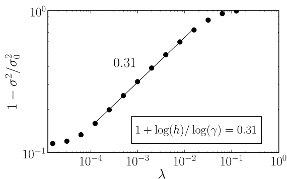
Figure 6.11: Evolution of 1 - I^2(\phi) with the diffusion scale \lambda , for a realization of the 1-D map with parameters \gamma = 1/2 and U = 0.14 . The fraction of the variance lost in the mixer varies as a power law with \lambda , whose exponent agrees very well with 1 + \log(h)/\log(\gamma) .
