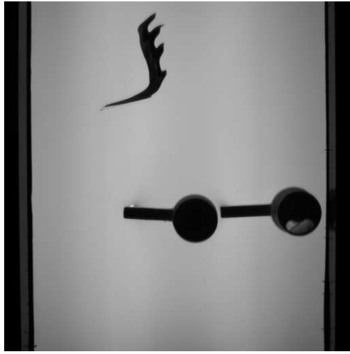
Figure 3.13: A dye blob initialized with no intersection with \mathcal{W}_s has been carried away downstream without being caught by the rods. Mixing is very inefficient for this initial condition.
