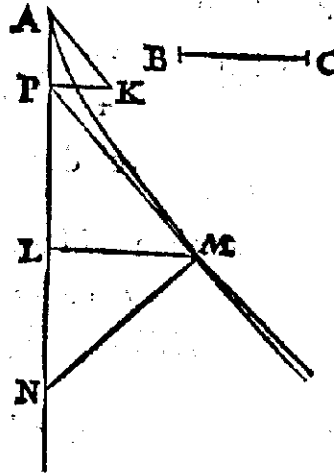
FIG. 10.3 – Geometria (1649), p. 147
