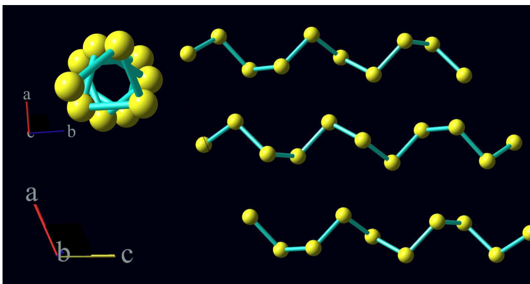
Figure 2.10: The proposed structure of fibrous sulfur from the model of Lind and Geller [60].
