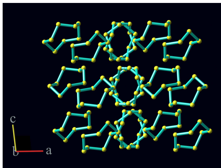
Figure 2.6: The structure of monoclinic sulfur projected along the crystal b -axis. The two possible orientations of one third of the molecules are reported by the two alternate position in the central rings. They transform one to the other by rotation around the C_4 axis of 45^\circ .
