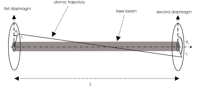
Fig. 7. Schematic view of an atom trajectory in the laser-atom interaction region.
