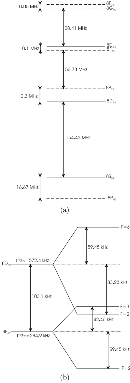
Fig. 12. (a) Fine structure and Lamb shifts of the 8S, 8P, 8D and 8F levels. The solid line corresponds to the levels which are excited with a two-photon transition from the metastable state. (b) Hyperfine structure of the 8D_{5/2} and 8F_{5/2} levels in hydrogen.
