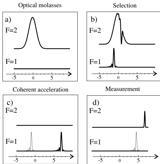
FIG. 1. Evolution of the velocity distribution (in v_r unit) during the experiment: (a) Initial velocity distribution; the atoms are in 5^2S_{1/2} , |F = 2, m_F = 0\rangle state. (b) Subrecoil selection; the atoms are transferred from 5^2S_{1/2} , |F = 2, m_F = 0\rangle to 5^2S_{1/2} , |F = 1, m_F = 0\rangle . (c) Coherent acceleration for N = 4 Bloch oscillations; the atoms are in 5^2S_{1/2} , |F = 1, m_F = 0\rangle . (d) Measurement of the final velocity class; the atoms are transferred from 5^2S_{1/2} , |F = 1, m_F = 0\rangle to 5^2S_{1/2} , |F = 2, m_F = 0\rangle .
