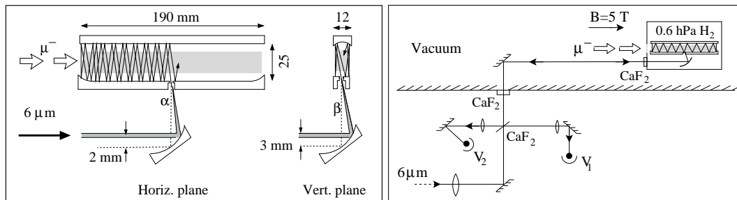
Fig. 7. (Left) Off-axis coupling into the 6\ \mu\text{m} cavity with \alpha = 40\ \text{mrad} and \beta = 60\ \text{mrad} . The 2-inch focal length of the parabolic gold coated mirror focuses the 6\ \mu\text{m} beam to the center of the 0.63\ \text{mm} diameter hole. (Right) Monitoring system for the 6\ \mu\text{m} cavity. Before entering the vacuum system 5% of the 6\ \mu\text{m} light is reflected by a 45^\circ \text{CaF}_2 plate and focused on a fast infrared detector V_1 . The transmitted pulse crosses the \text{CaF}_2 vacuum and target windows and enters the cavity. Part of the light escaping from the entrance hole travels back on the same axis as the incoming light and is detected with a second infrared detector V_2 . V_1 and V_2 are monitoring respectively the input pulse ( 6\ \mu\text{m} production) and the time distribution inside the cavity.
