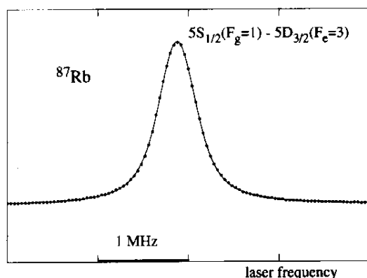
Fig. 2. Lineshape of the 5S_{1/2}(F_g=1) - 5D_{3/2}(F_e=3) hyperfine component in ^{87}\text{Rb} . The experimental points are fitted with a Voigt profile.
