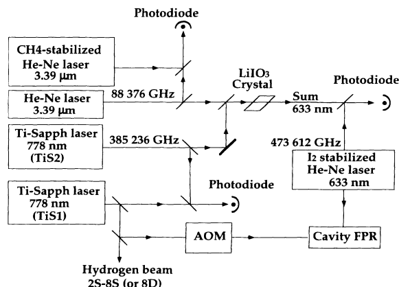
FIG. 1. Experimental setup for the frequency comparison between the 2S\text{-}8S/8D transition and the standard lasers.
