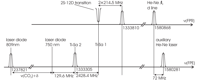
Fig. 18. Example of the position of the laser frequencies with respect to the FPR and FPE cavities during the measurements of the 2S–12D transitions. The fringe 1 580 868 of the FPR cavity is locked on the d line of the He–Ne/ \text{I}_2 standard laser. The first titanium sapphire laser (Ti-Sa1) is locked on the fringe 1 333 810 of the FPR cavity with an offset of 2 \times 214.5 MHz. The 809 nm laser diode, the second titanium sapphire laser (Ti-Sa2) and the auxiliary He–Ne laser are respectively locked on the fringes 1 237 821, 1 333 305 and 1 580 281. The laser diode at 750 nm is frequency shifted by \nu(\text{CO}_2) + \delta with respect to the one at 809 nm.
