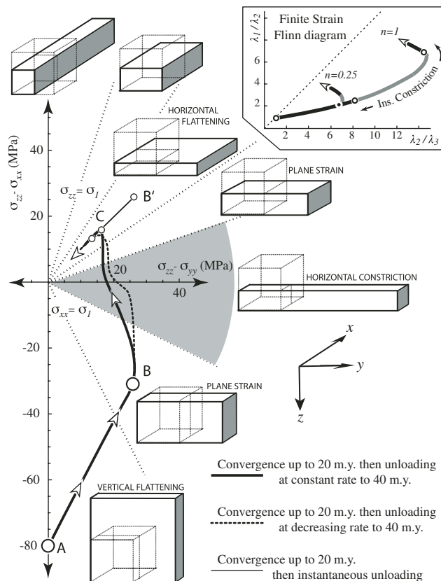
Figure 1. Warm and buoyant continental lithosphere is submitted to a tectonic force that drives convergence at initial strain rate of 5 \times 10^{-15} \text{ s}^{-1} . A: Driving force is constant for 20 m.y. before it decreases progressively to zero over a 20 m.y. period. Three unloading histories are considered. B: Each tectonic history results in slightly different evolution of vertical geometry of continental lithosphere.
