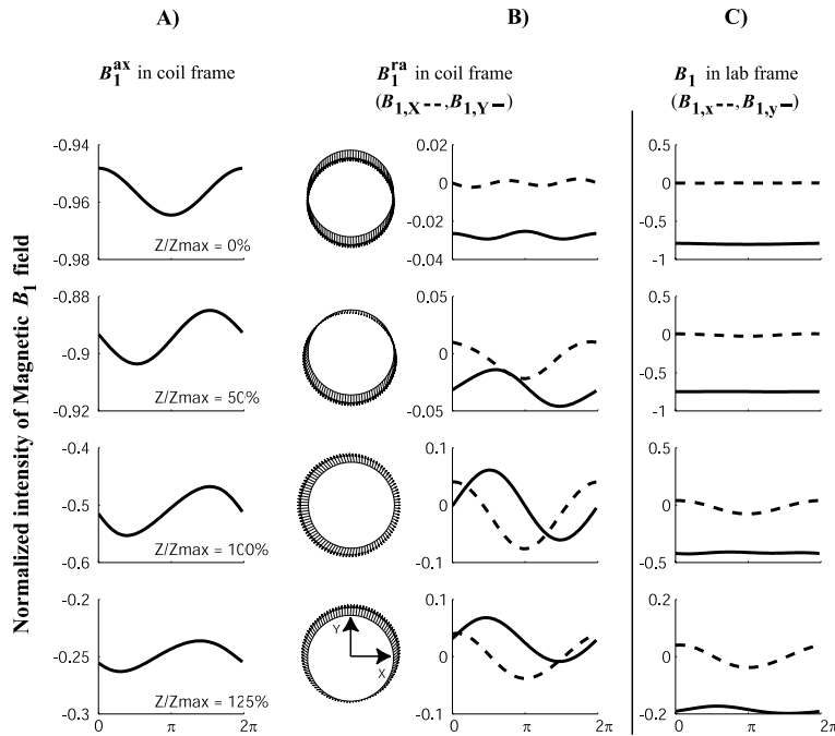
FIG. 8.2 – Set of figures \rho = 0.5 \text{ mm} : Magnetic field vectors calculated in the empty coil, and displayed around circular rings of diameter 1 mm.
